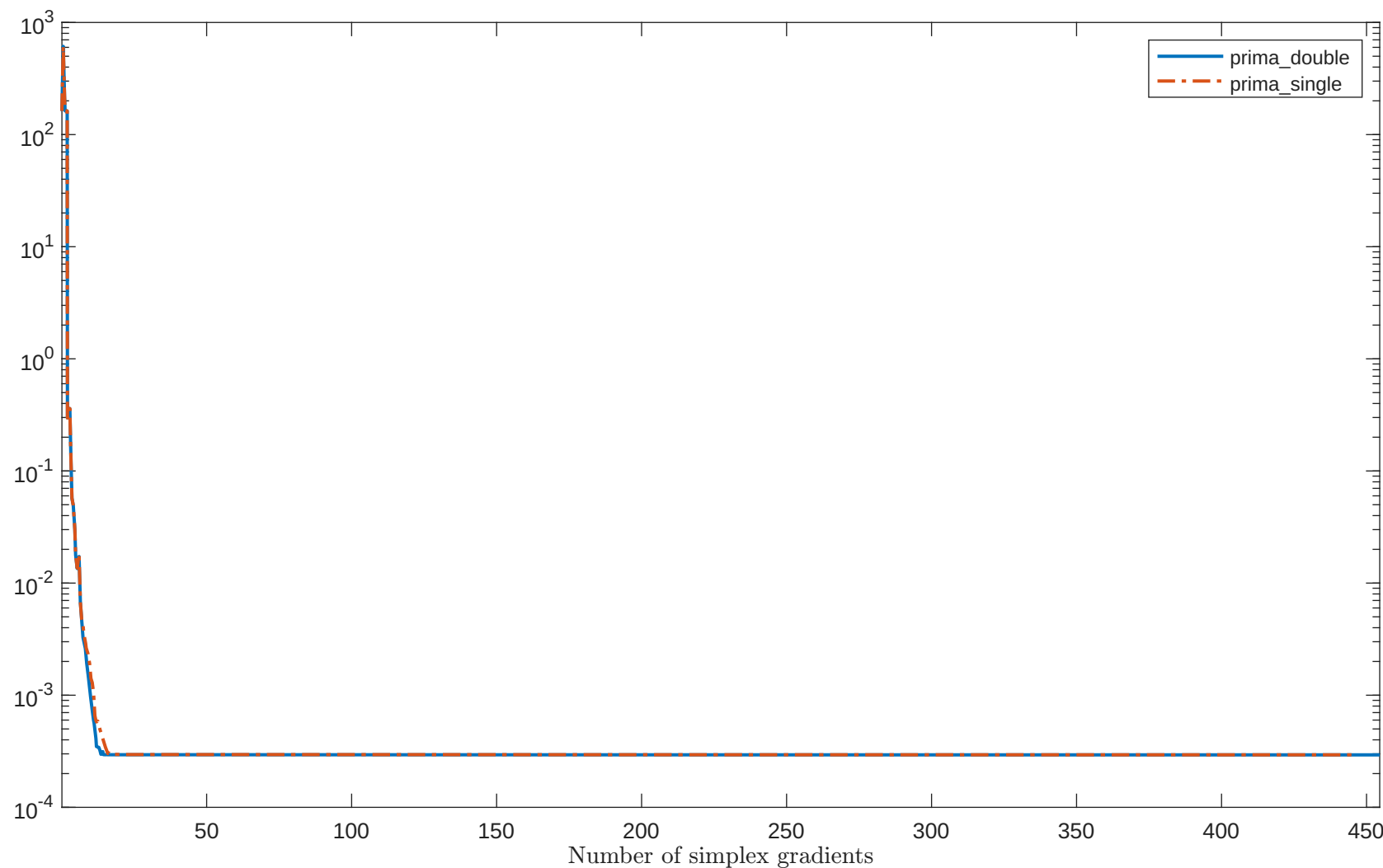
Solving "PENALTY2" with "plain" feature
