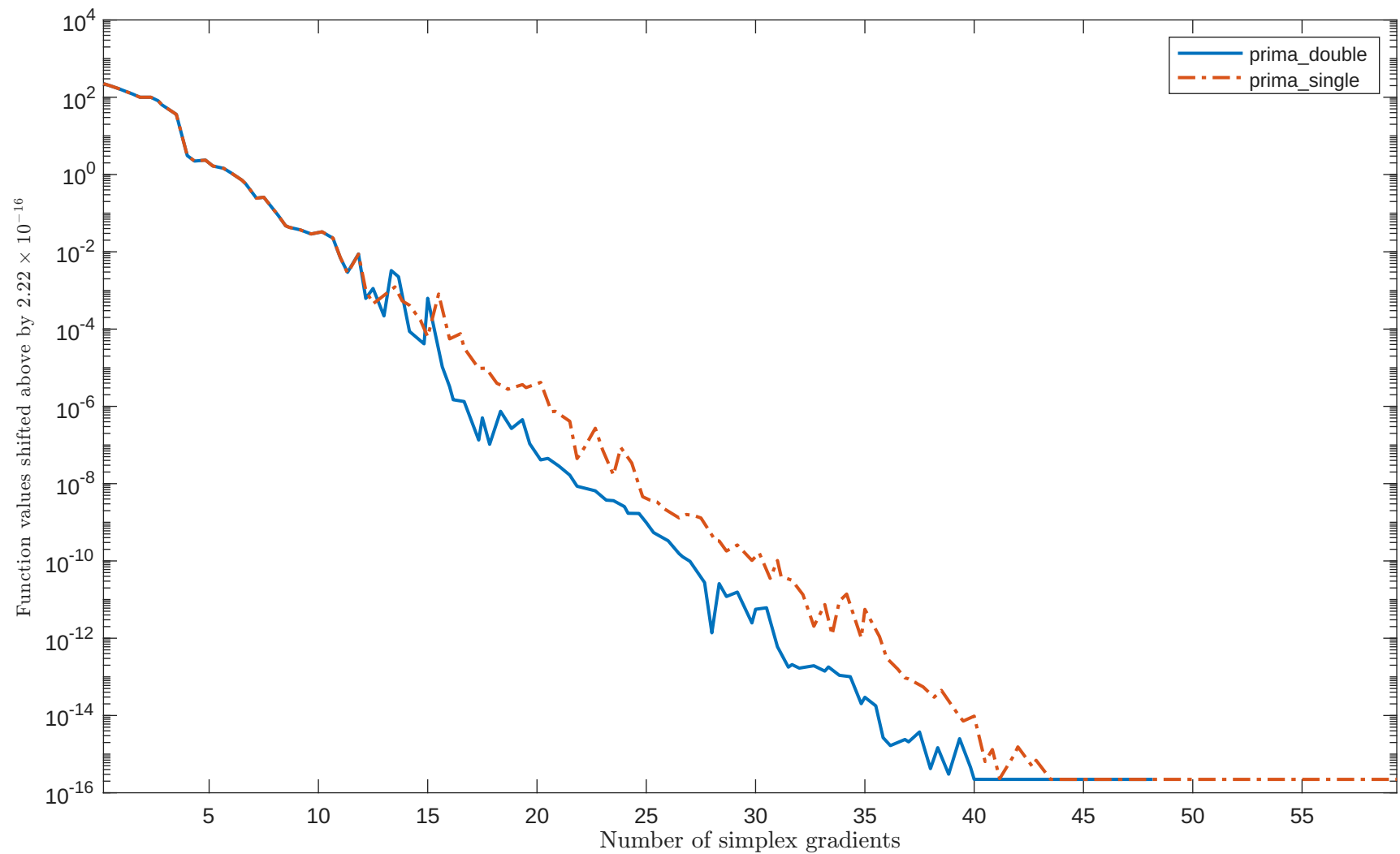
Solving "POWER" with "plain" feature
