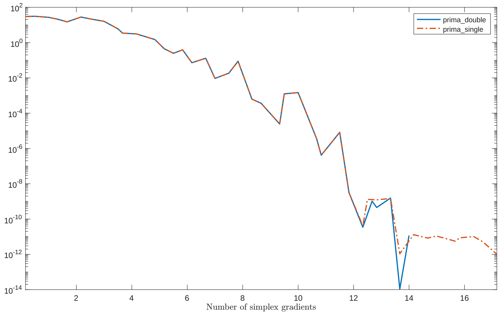
Solving “QING” with “plain” feature
