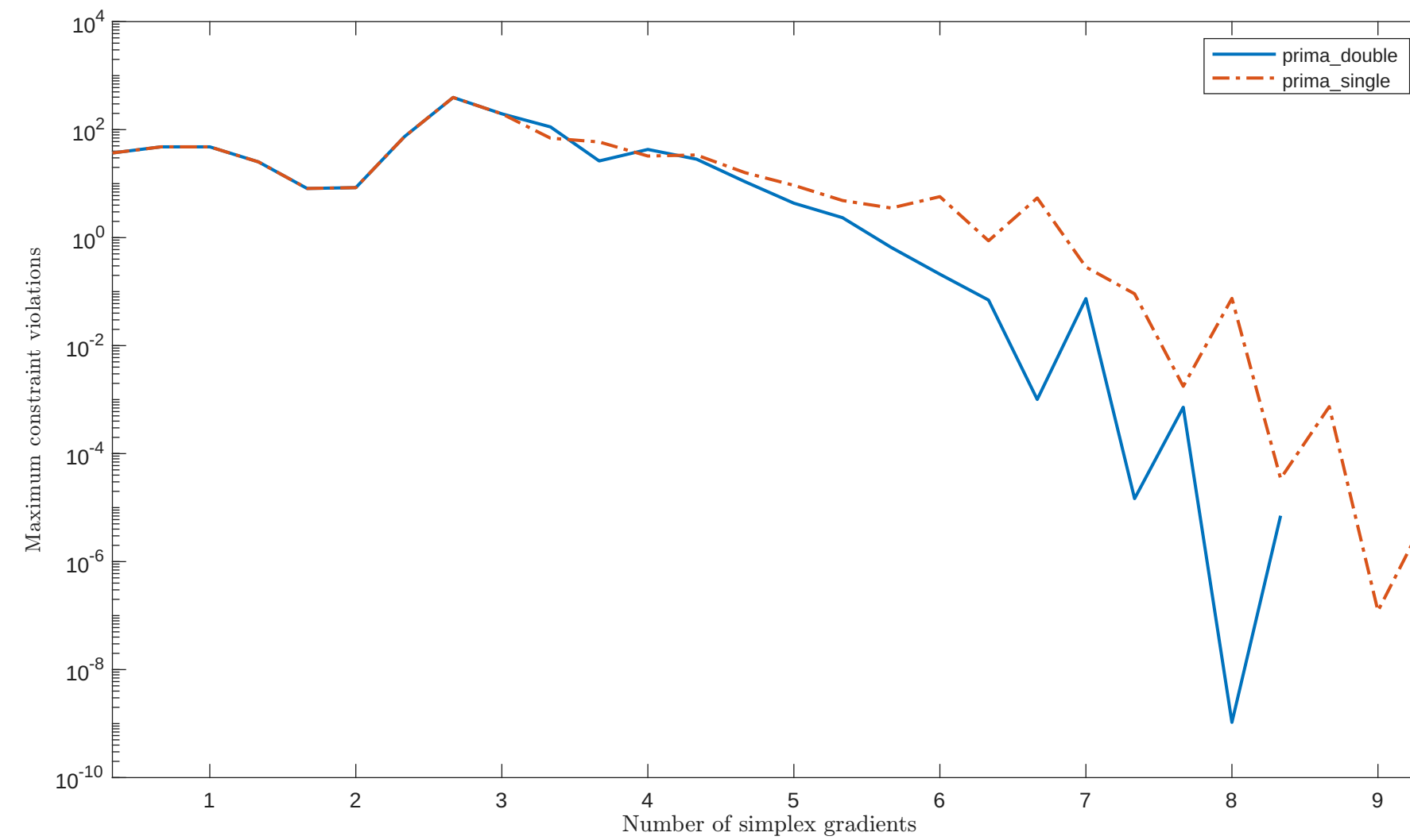
Solving "ROSEPETAL" with "plain" feature
