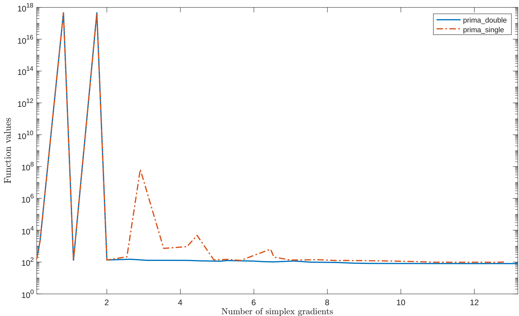
Solving “SBRYBND” with “plain” feature
