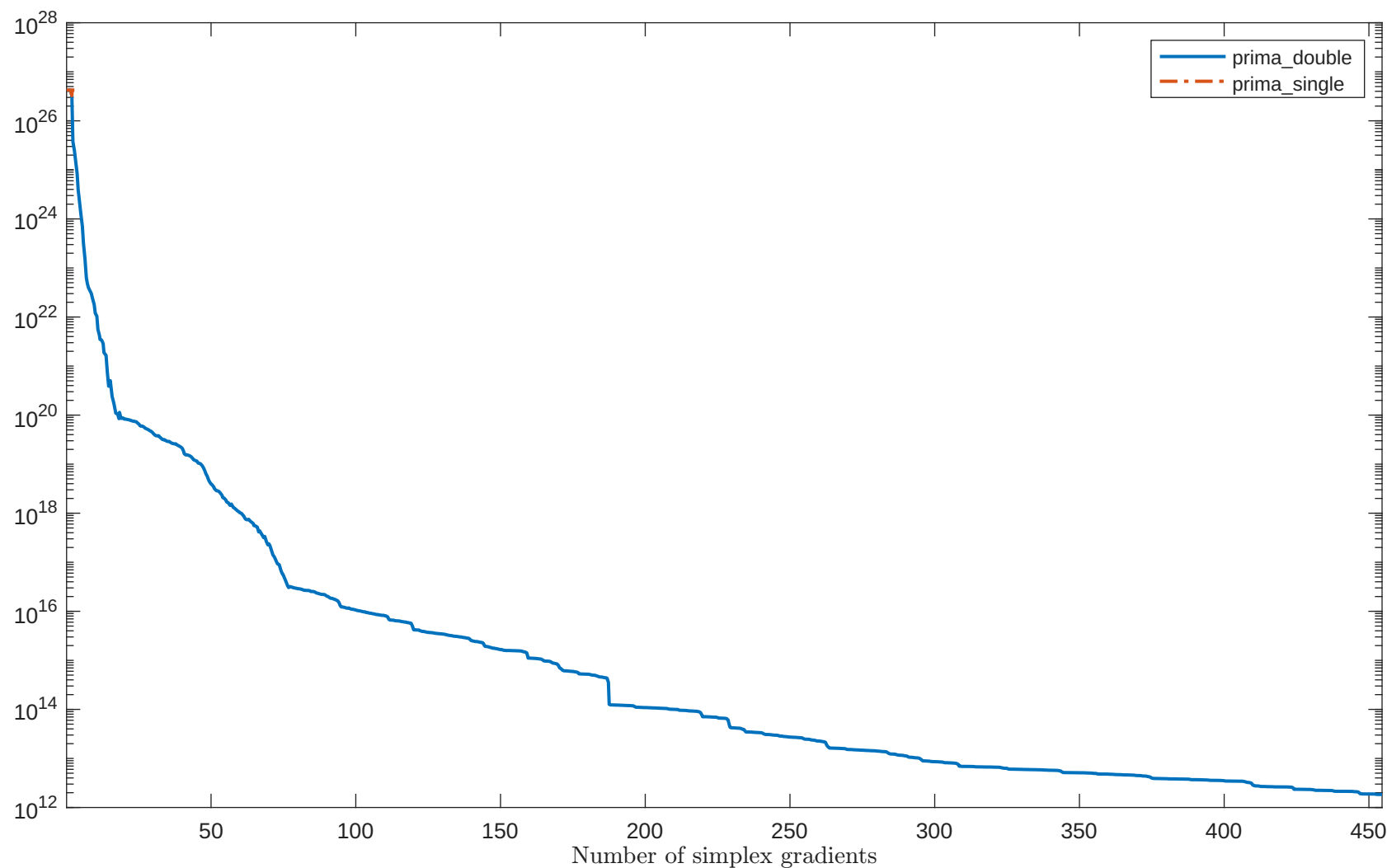
Solving "SCURLY10" with "plain" feature
