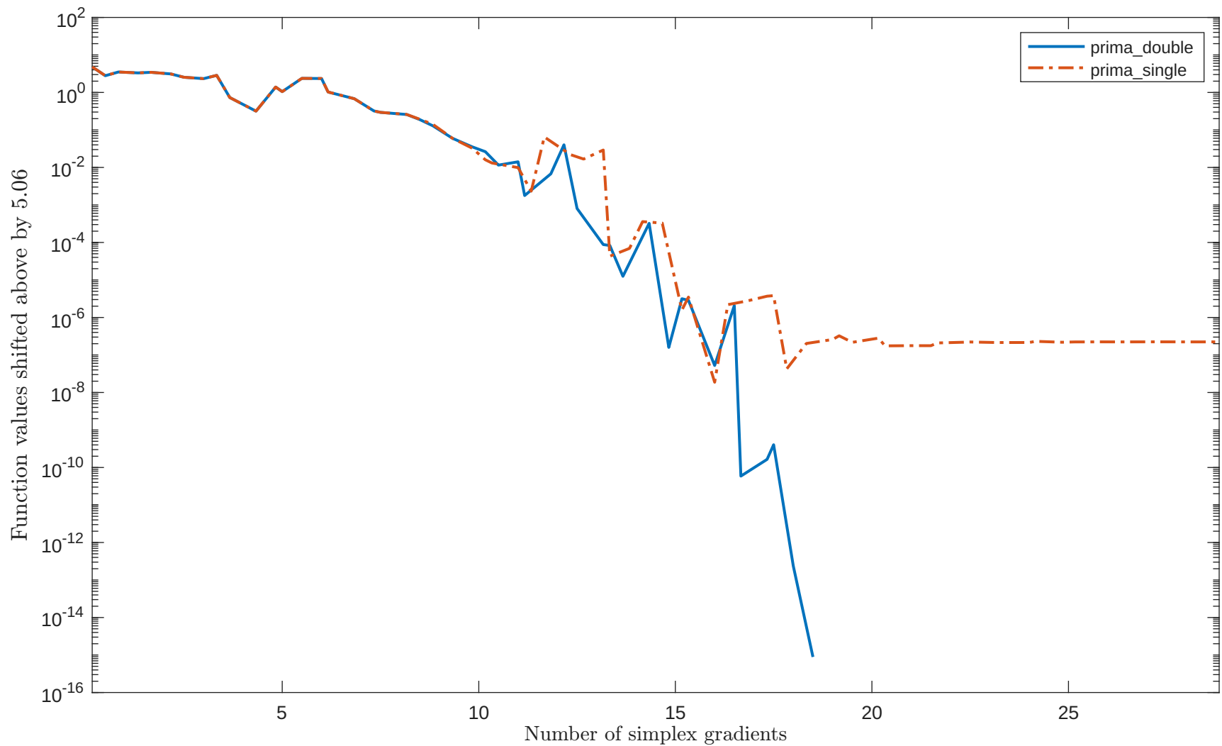
Solving "SENSORS" with "plain" feature
