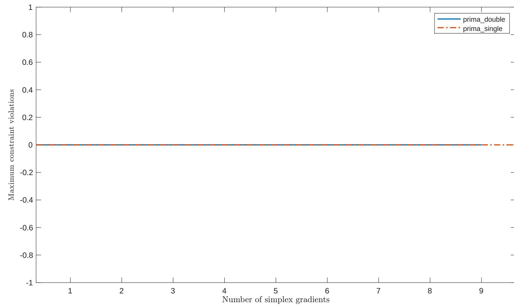
Solving "SIMBQP" with "plain" feature
