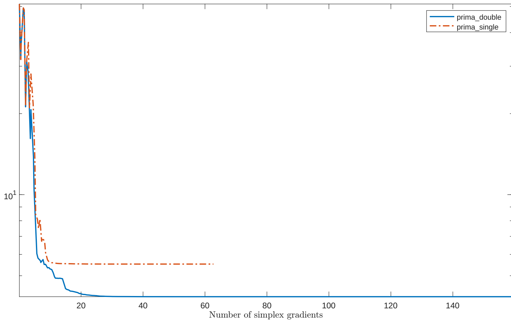
Solving “TRIGON2” with “plain” feature
