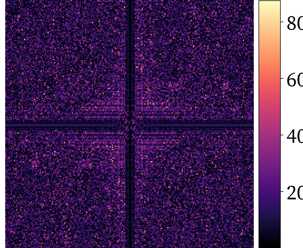
(e) \Delta\text{freq}(\text{mid}+\text{high})=+6.00\%
