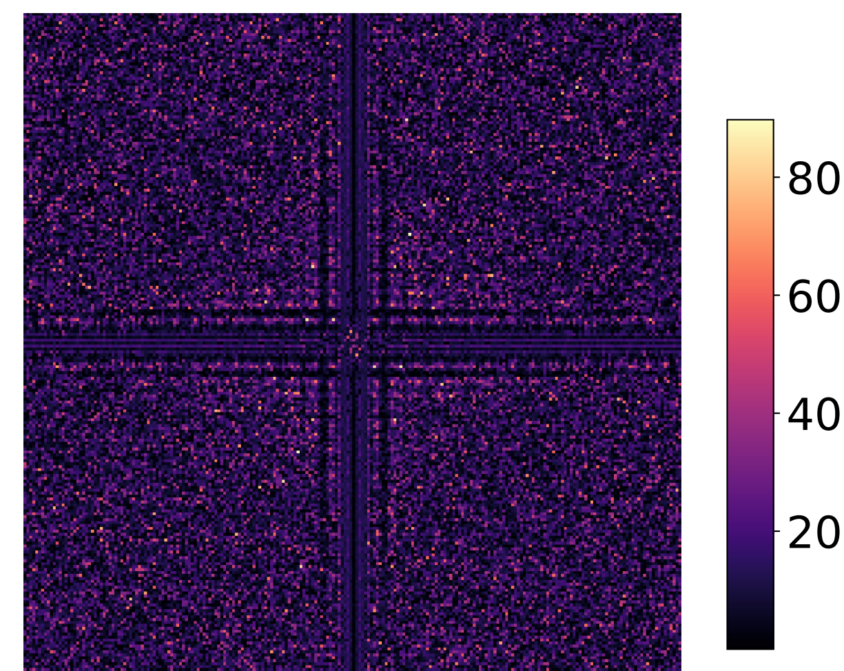
\Delta\text{Freq}(\text{Mid}+\text{High})=+4.21\%
