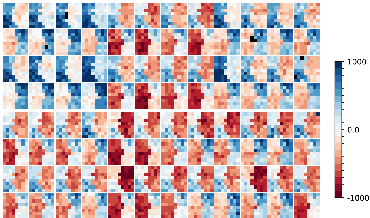
All channels computed time offsets (ps)
