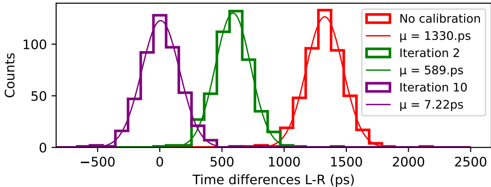
Channel pair (3580, 847) time differences
