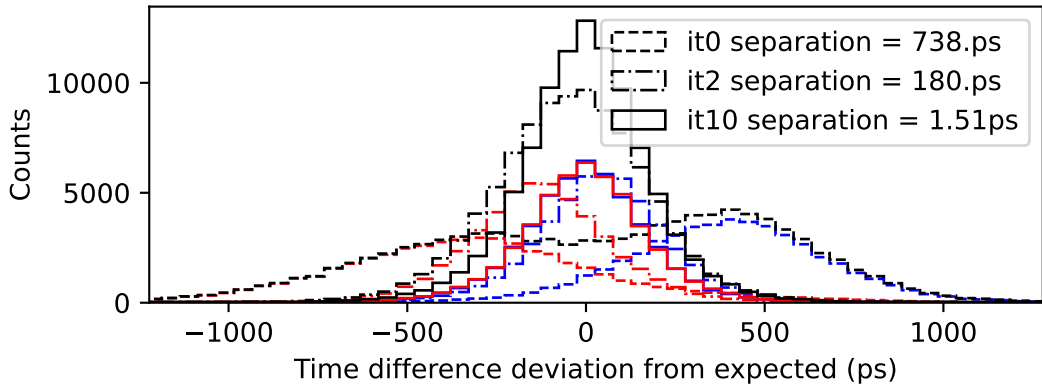
Time difference deviation from expected, channel 3527
