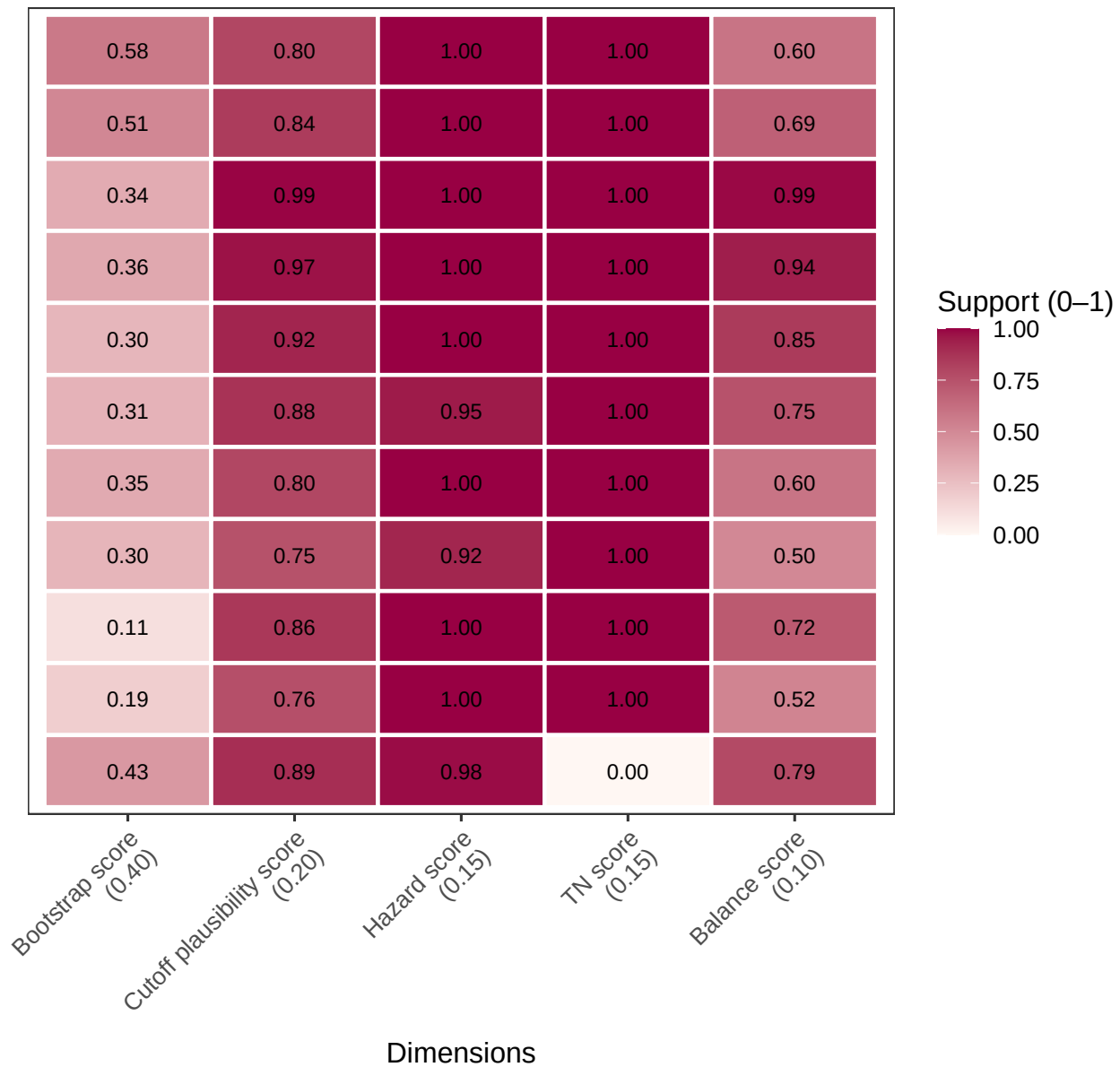
StaBiCut mean composite stability score
