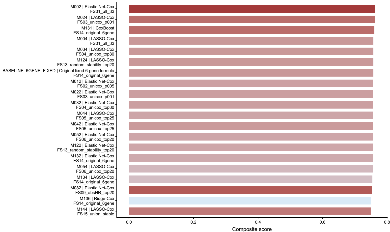
Top 20 Phase 3A model combinations
