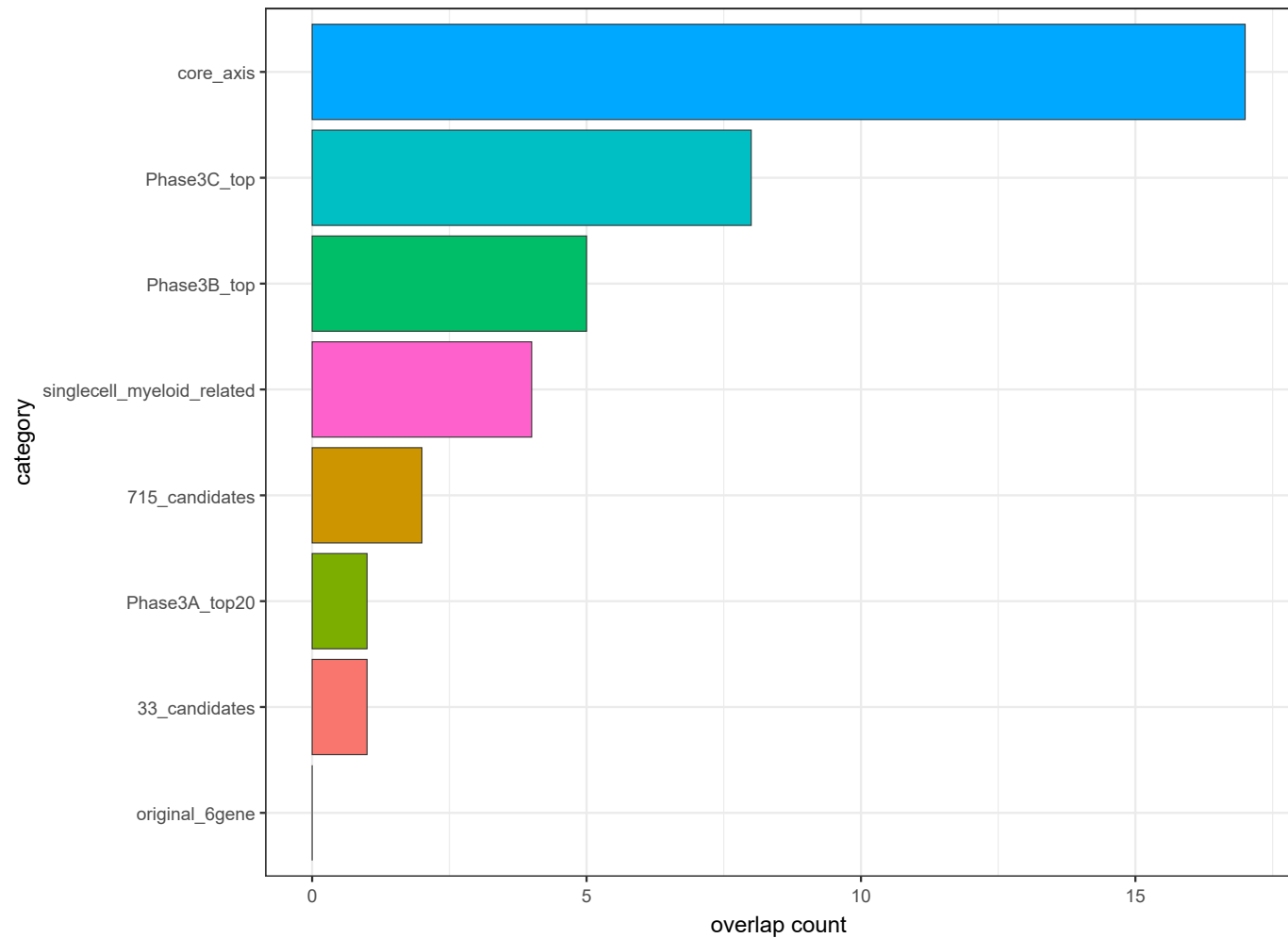
Overlap of PPI hub genes with PRFT-related modules
