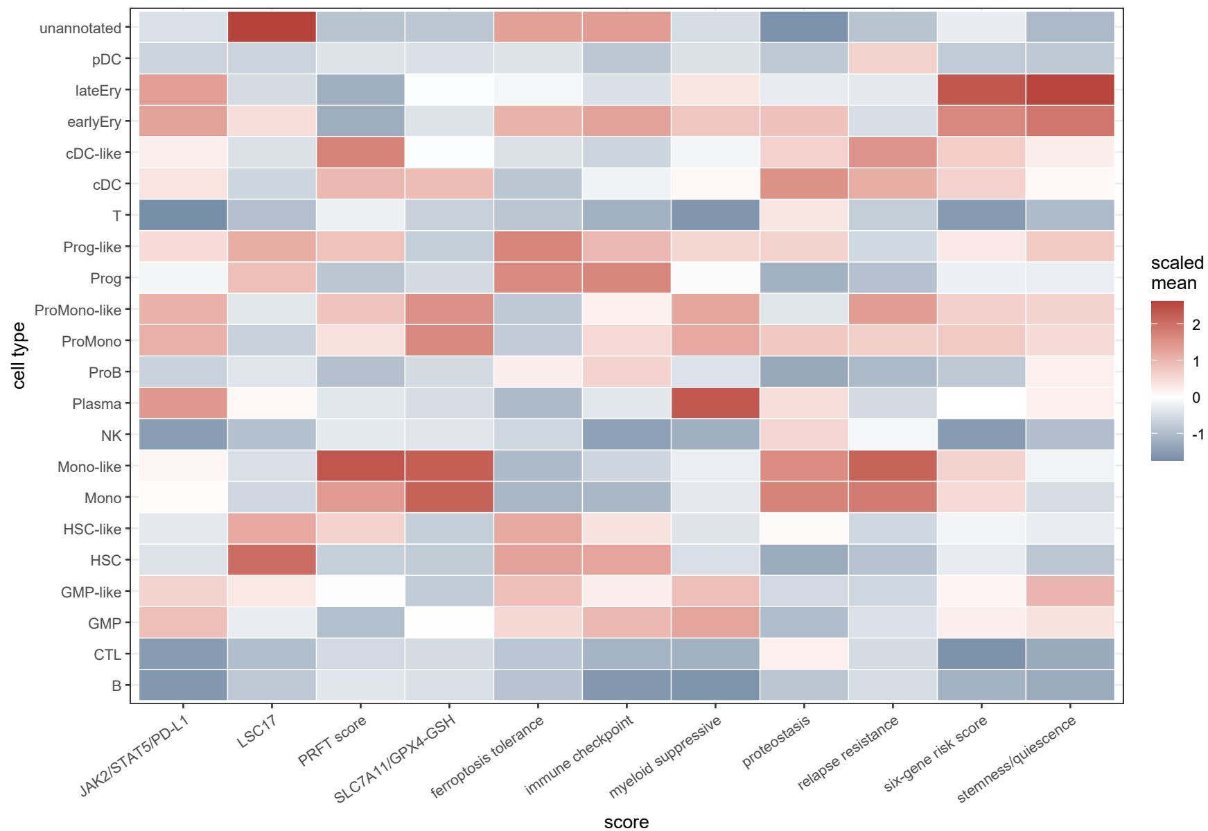
Scaled PRFT-related scores by cell type
