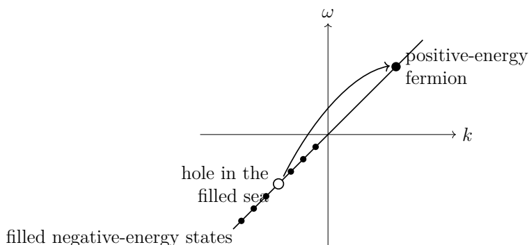
Figure 5.8: The filled negative-energy sea and an excitation formed by promoting one fermion to positive energy.
