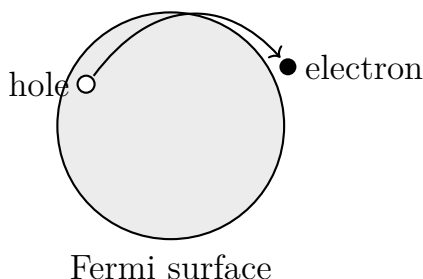
Figure 5.5: A low-energy fermionic excitation promotes an electron through the Fermi surface and leaves a hole behind.
