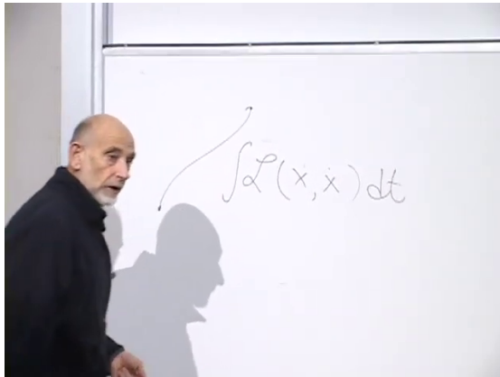
Figure 10.1: Action integral for a particle trajectory.
