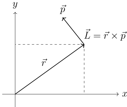
Figure 7.1: For a particle at position \vec{r} with momentum \vec{p} , the angular momentum \vec{L} = \vec{r} \times \vec{p} is perpendicular to their plane.
