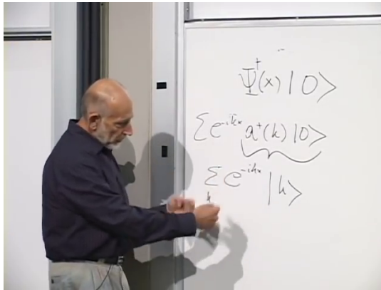
Figure 3.3: The formal position-space state \Psi^\dagger(x)|0\rangle expanded in one-particle momentum states.
