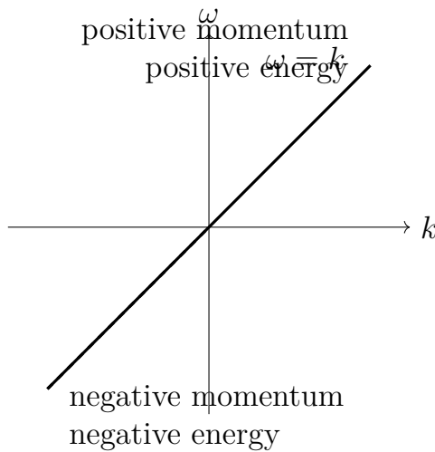
Figure 5.7: The one-branch spectrum \omega = k , with its negative-energy half at k < 0 .
