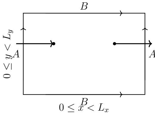
Figure 3.6: A two-dimensional periodic space: edges carrying the same label are identified, so a particle crossing one edge reappears at the corresponding point on the opposite edge.
