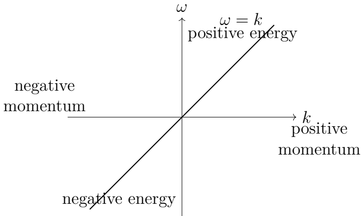
Figure 6.1: The massless right-moving dispersion \omega = k contains positive- and negative-energy branches.
