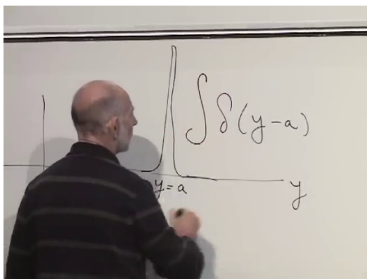
Figure 4.1: Unit-area delta-function spike centered at y = a .
