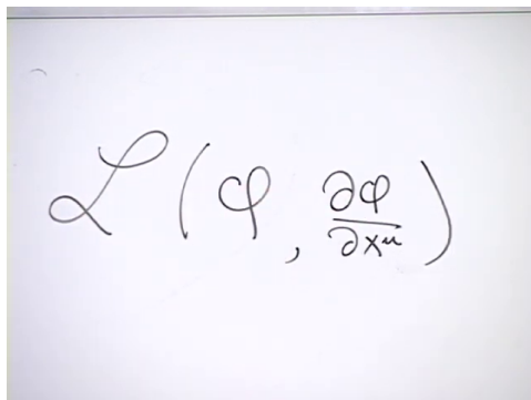
Figure 10.2: Dependence of the field Lagrangian on the field and its spacetime derivatives.
