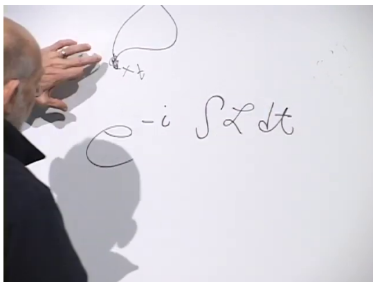
Figure 10.4: Complex phase associated with a particle path.
