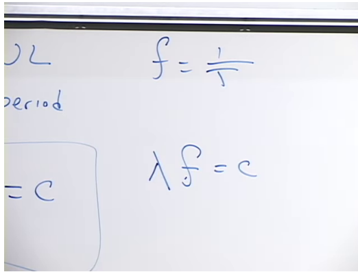
Figure 1.4: For a light wave, f = 1/T and \lambda f = c .
