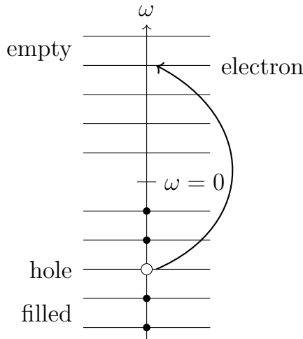
Figure 6.2: Promoting an occupied negative-energy electron produces a positive-energy electron and leaves a hole in the filled sea.
