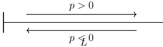
Figure 2.7: Reflection at the ends of a finite segment reverses the momentum of a traveling wave.
