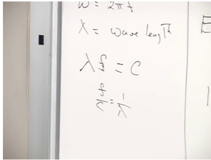
Figure 2.1: For light, \lambda f = c and f/c = 1/\lambda , the relations used to obtain |\vec{p}_\gamma| = h/\lambda .
