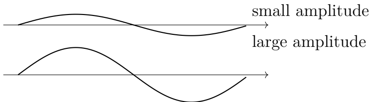
Figure 2.2: Waves with equal wavelength and frequency but different amplitudes.
