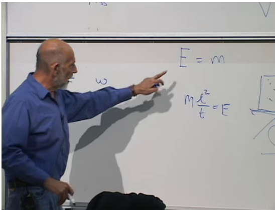
Figure 1.7: In units with c = 1 , the rest energy of a massive object at rest is E = m .
