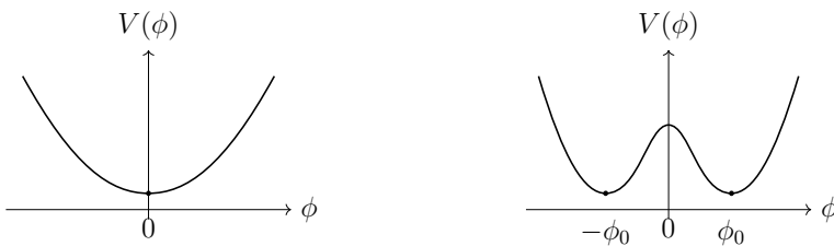
Figure 6.9: Even potentials may have a centered minimum or two symmetry-related nonzero minima.
