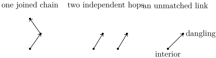
Figure 10.7: Joined, independent, and unmatched selections of neighboring links.
