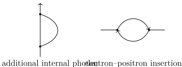
Figure 10.16: Two higher-order QED structures that add elementary vertices and further powers of e .
