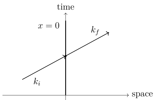
Figure 4.7: A particle of momentum k_i scatters from a target fixed at x = 0 and emerges with momentum k_f .
