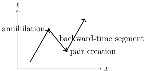
Figure 10.8: A backward-time segment read forward as pair creation and annihilation.
