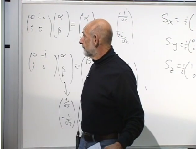
Figure 8.3: Normalized \sigma_y eigenvectors alongside the three spin-one-half matrices.
