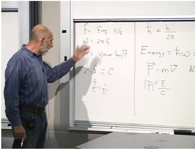
Figure 2.3: Wave definitions and the photon and nonrelativistic momentum relations compared by their domains of validity.
