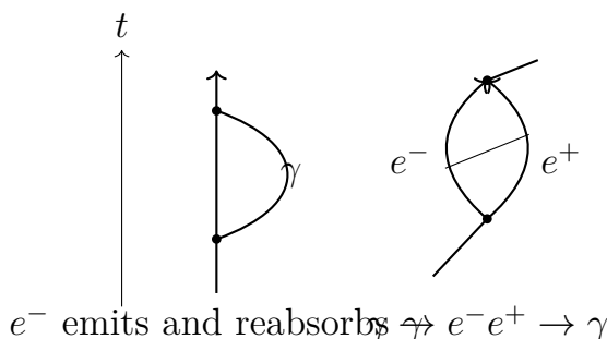
Figure 10.11: An electron self-emission contribution and a photon history containing an electron-positron pair.
