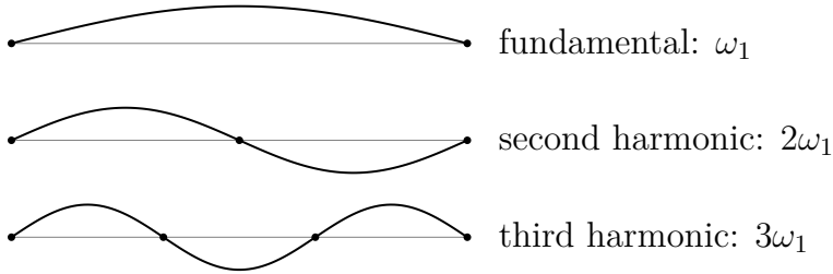
Figure 2.11: The string fundamental and its second and third harmonics, with zero, one, and two interior nodes.
