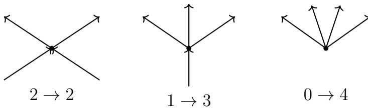
Figure 10.12: Three local orientations of a four-leg interaction vertex.
