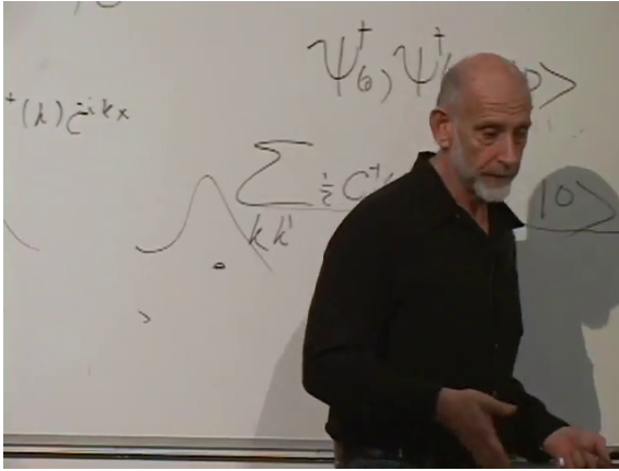
Figure 5.2: Localized one-particle wavefunctions and the two-creation-operator state used to test fermionic exclusion.
