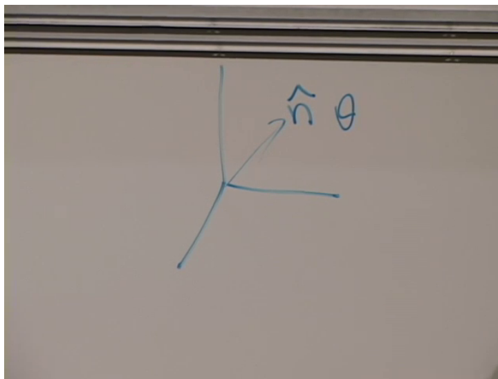
Figure 3.1: An axis \hat{n} and an angle \theta specify a spatial rotation.
