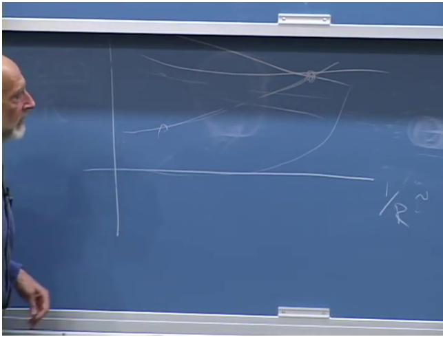
Figure 10.9: The board's qualitative coupling plot: the strong curve falls, the electroweak curves evolve slowly toward it, and gravity rises steeply near the far ultraviolet.
