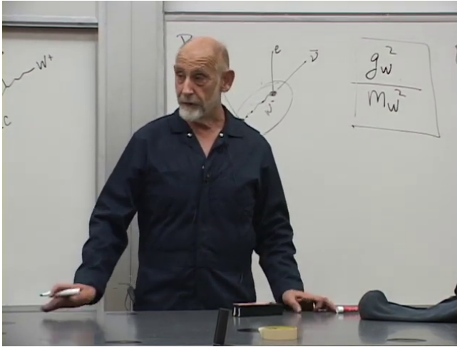
Figure 6.5: The beta-decay topology beside the boxed low-energy estimate g_w^2/m_W^2 .
