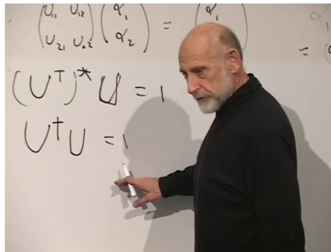
Figure 3.3: The spinor rotation matrix obeys U^\dagger U = 1 .
