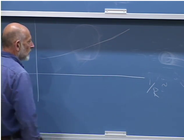
Figure 10.7: The QED effective charge rises slowly as the horizontal scale 1/R , and therefore the probing energy, increases.
