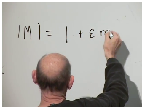
Figure 4.2: The first-order determinant expansion as it begins on the board.
