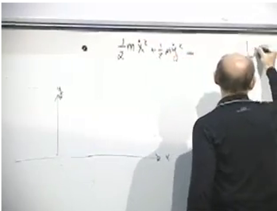
Figure 3.10: The two-coordinate kinetic energy and near-Earth setup at 01:15:15. The stable board content is T = \frac{1}{2}m\dot{x}^2 + \frac{1}{2}m\dot{y}^2 ; the potential is completed immediately afterward.
