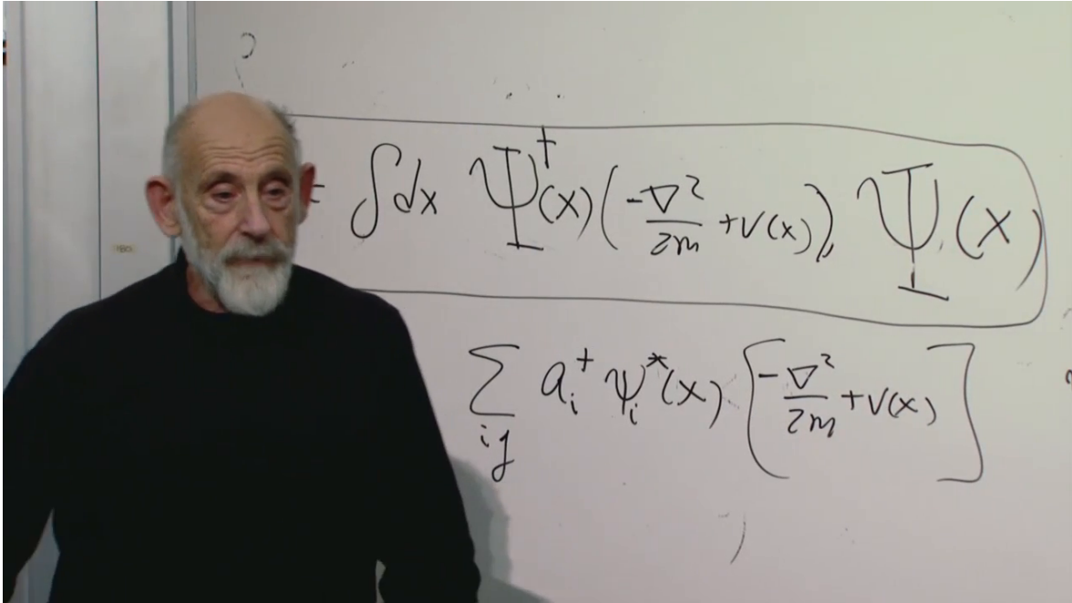
Figure 7.4: The field Hamiltonian emphasized on the board, with the mode-expansion proof beginning below it. The live frame is retained as evidence; Equations (7.33)–(7.39) restore the complete algebra.
