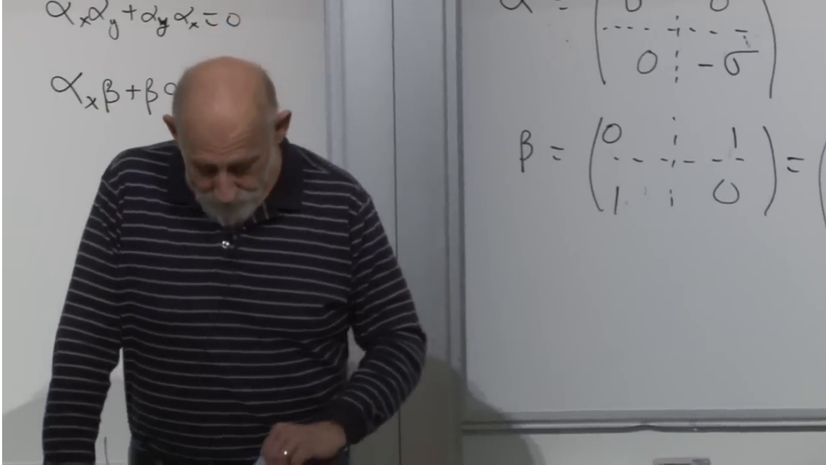
Figure 10.6: The board's 4 \times 4 block representation. The upper equations record the required anti-commutators; the full matrices are typeset in Eq. (10.44).
