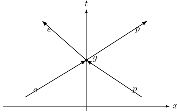
Figure 9.2: A clean reconstruction of the local scattering picture. The vertex is shorthand for the operator in Eq. (9.20), not a classical collision law.
