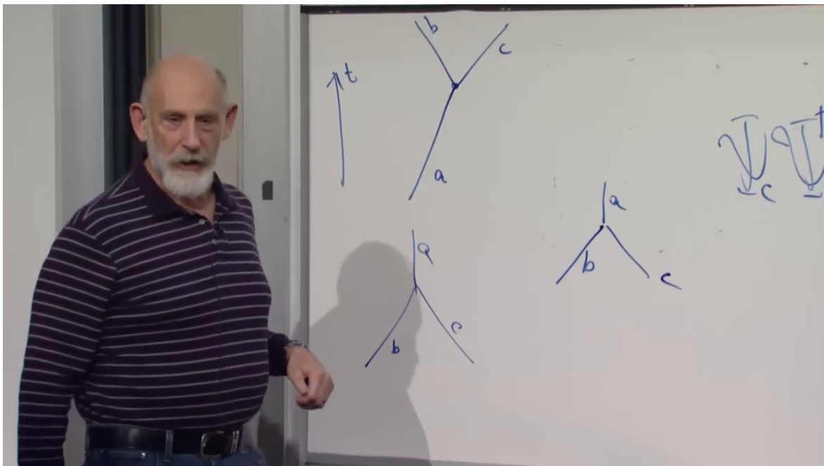
Figure 9.3: The two orientations of the elementary A \leftrightarrow B + C vertex on the board. Juxtaposing them is the visual shorthand for the second-order process in Eq. (9.28).
