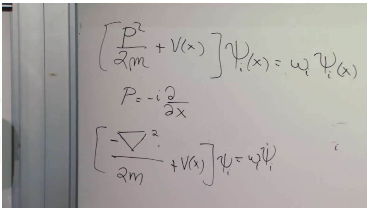
Figure 7.3: The board passage from p^2/(2m) + V(x) to the differential form of the one-particle Schrodinger eigenvalue equation. Equation (7.31) is its cleaned reconstruction.
