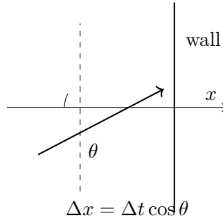
Figure 5.5: Photon momentum incident on a wall at angle \theta , the geometry used to derive radiation pressure.
