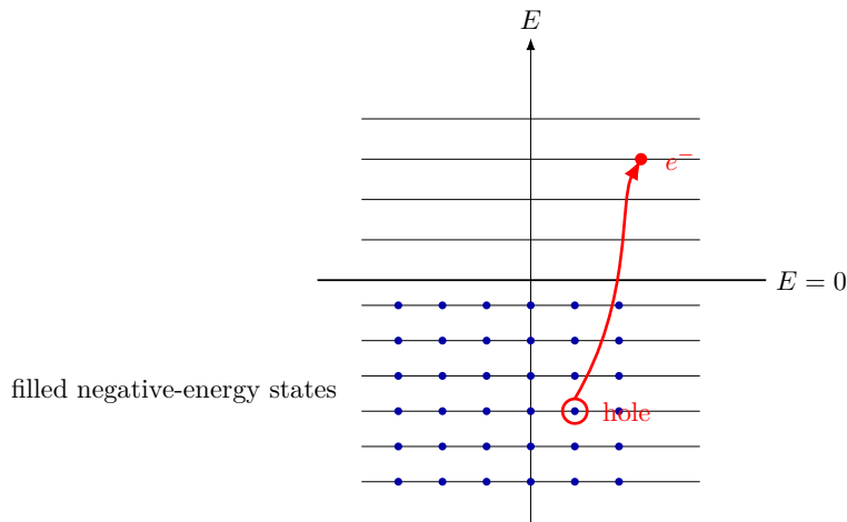
Figure 10.8: A clean reconstruction of excitation above a filled sea: promoting one negative-energy electron leaves a positive-energy hole.
