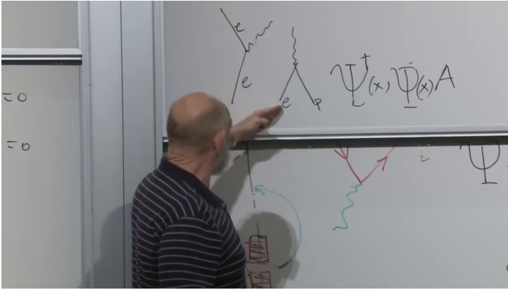
Figure 10.10: The board juxtaposes electron emission, pair annihilation, and the schematic interaction \psi^\dagger \bar{\psi} A . Different selections from the same field operators generate the different channels.
