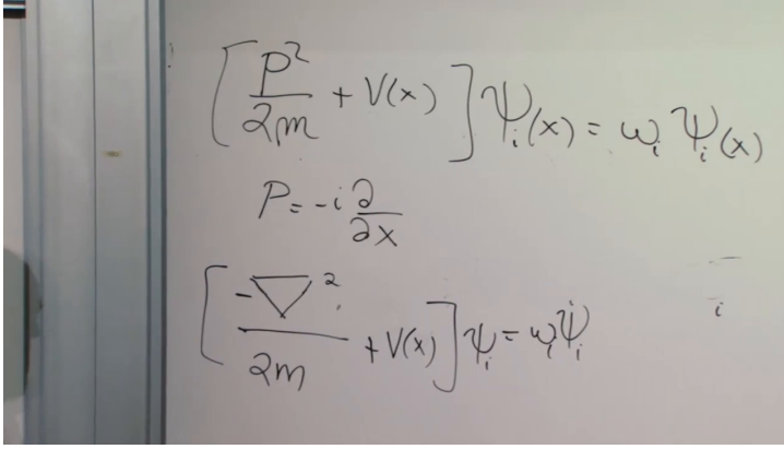
Figure 7.3: The board passage from p^2/(2m) + V(x) to the differential form of the one-particle Schrodinger eigenvalue equation. Equation (7.32) is its cleaned reconstruction.
