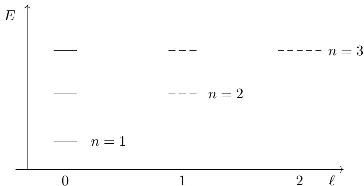
Figure 4.2: The first three ideal Coulomb shells combine orbital multiplets of equal principal energy: one state in the first shell, 1 + 3 in the second, and 1 + 3 + 5 in the third.
