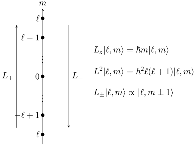
Figure 3.1: An integer orbital angular-momentum multiplet. L_+ and L_- change m by one, while L^2 remains \hbar^2 \ell(\ell + 1) throughout the multiplet.
