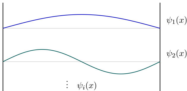
Figure 7.2: A clean reconstruction of the qualitative box sketch. The vertical offsets merely separate the two wavefunctions for display.
