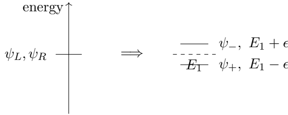
Figure 8.3: The board logic of the tunnel splitting. The approximate left and right states are nearly degenerate, but the exact symmetric and antisymmetric eigenstates are split by a small amount 2\epsilon .
