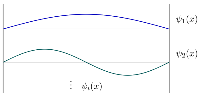
Figure 6.3: A clean reconstruction of the qualitative box-mode sketch. The vertical displacement separates the eigenfunctions for readability and is not an additional physical coordinate.
