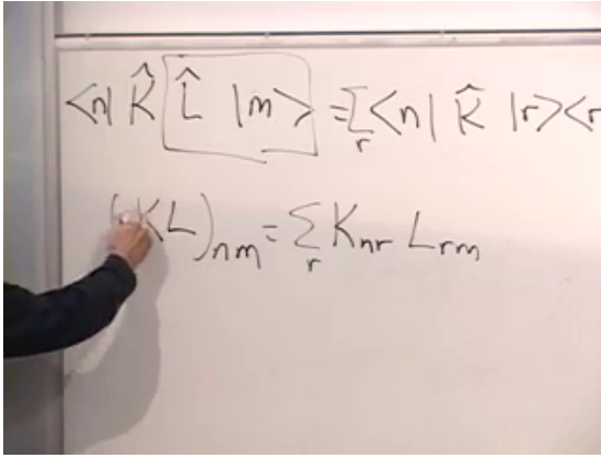
Figure 3.5: Insertion of a complete basis between two operators.
