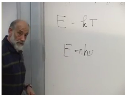
Figure 9.2: Planck's discrete energy rule, whose interpretation Einstein extended from material emitters to radiation itself.
