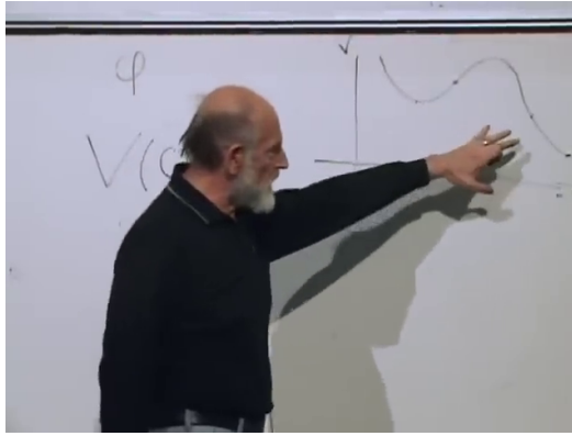
Figure 7.2: Qualitative scalar potential V(\phi) showing that different field values carry different potential energies.
