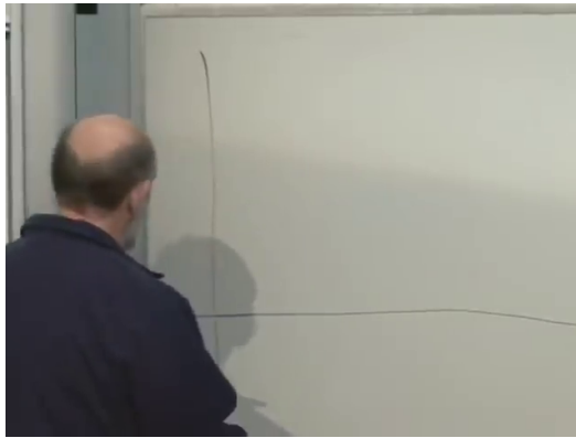
Figure 3.3: Axes for comparing matter and radiation energy density as functions of the scale factor.
