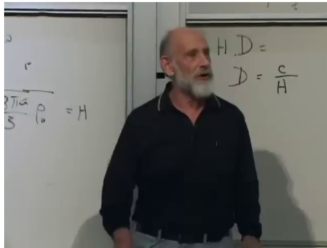
Figure 7.1: Cosmic horizon relation D = c/H in de Sitter expansion.
