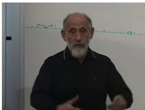
Figure 4.1: One-dimensional line used to picture an expanding metric.
