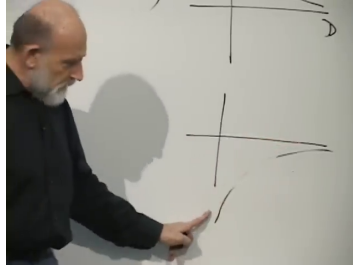
Figure 2.4: Qualitative comparison of 1/D and -1/D for the sign of gravitational potential energy.
