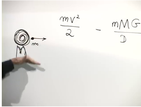
Figure 2.3: Total Newtonian energy for a radially moving test mass: kinetic term minus gravitational potential.
