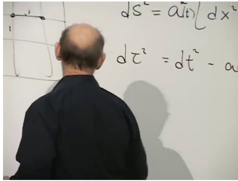
Figure 2.1: Comoving grid sketch and spacetime interval with a time-dependent scale factor.
