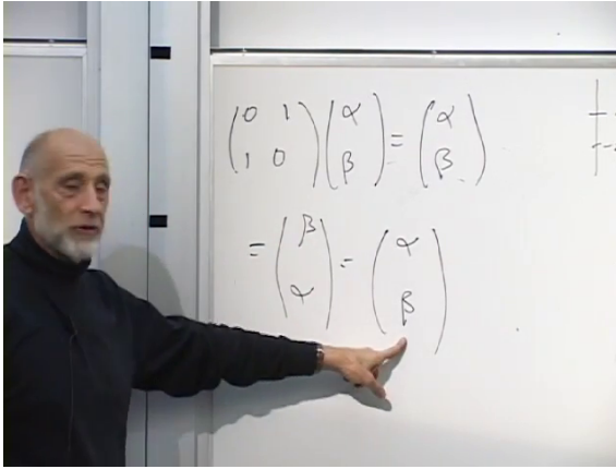
Figure 8.2: For eigenvalue +1 , \sigma_x exchanges the two components, requiring \alpha = \beta .
