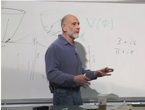
Figure 8.3: The board's radial potential sketches. The potential is symmetric under rotations of the internal field value, even though the field itself need not sit at the origin.
