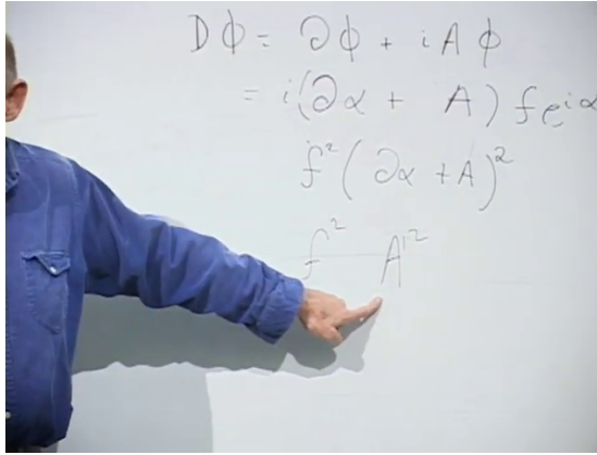
Figure 9.3: The board isolates the f^2 A^2 term that signals a gauge-boson mass after the phase has been absorbed.
