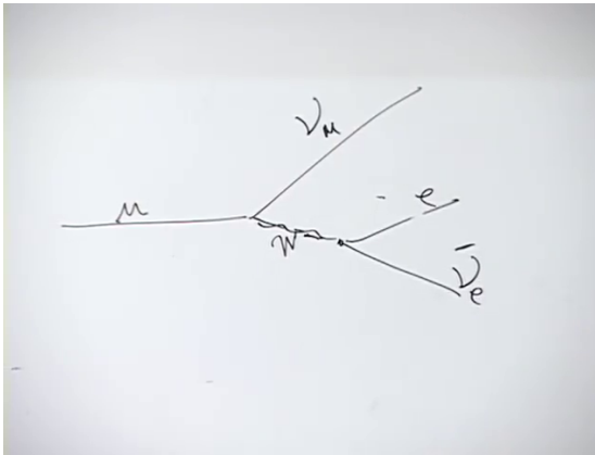
Figure 5.5: Muon decay through a virtual charged weak boson.
