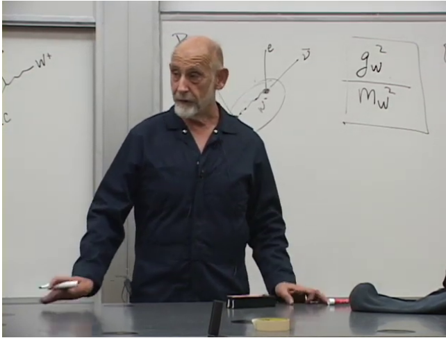
Figure 6.5: The beta-decay topology beside the boxed low-energy estimate g_w^2/m_W^2 .
