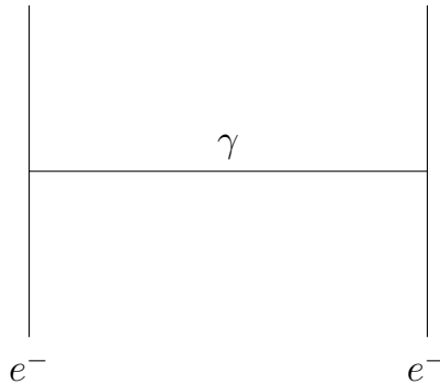
Figure 1.7: Topological schematic of photon exchange, giving the quantum-field-theoretic description of the Coulomb interaction.
