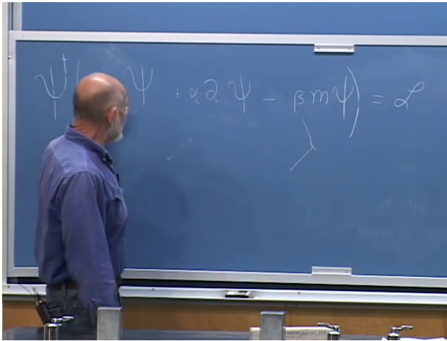
Figure 10.1: The Dirac equation and Lagrangian in the older \alpha, \beta notation. The board is being used structurally rather than as a fixed sign convention.
