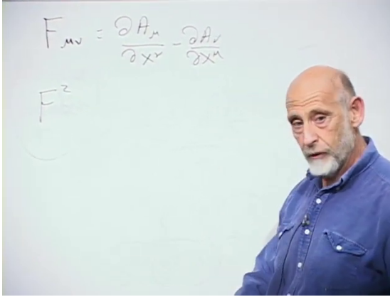
Figure 9.1: The field-strength definition and the board's F^2 shorthand for the derivative energy of the gauge field.
