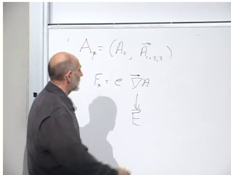
Figure 5.1: The electromagnetic four-potential and its derivative relation to the field.
