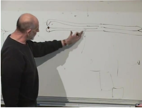
Figure 4.5: Color flux bundled into a long tube between a quark and an anti-quark.
