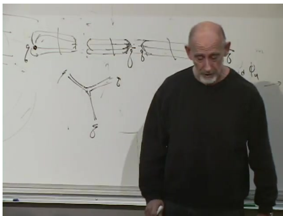
Figure 4.7: A three-pronged color-flux junction for a baryon, below the meson string-breaking sketch.
