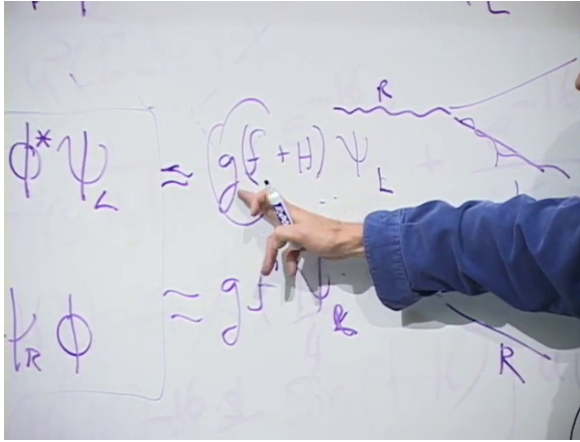
Figure 9.7: The board restores the Higgs fluctuation inside the Yukawa term: the constant part produces the fermion mass and the fluctuating part produces Higgs emission or absorption.
