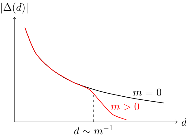
Figure 6.3: A clean schematic of the board argument. It is not an exact formula for a four-dimensional propagator; it isolates the mass-controlled range.
