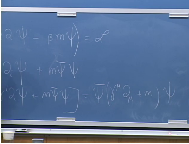
Figure 10.2: The covariant rewrite: \bar{\psi} = \psi^\dagger \gamma^0 , \gamma^i = \beta \alpha^i , and the compact Dirac Lagrangian.
