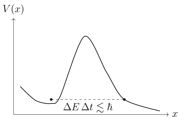
Figure 6.7: A readable reconstruction of the barrier and equal-energy points.
