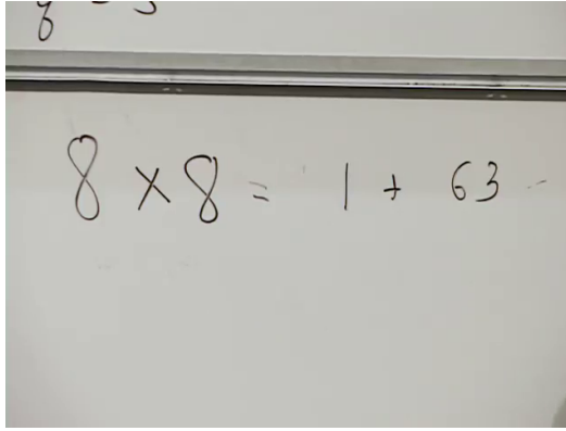
Figure 4.4: The board's two-gluon state count: one singlet among sixty-four states.
