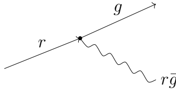
Figure 2.6: A red quark becomes green while emitting an r\bar{g} gluon.
