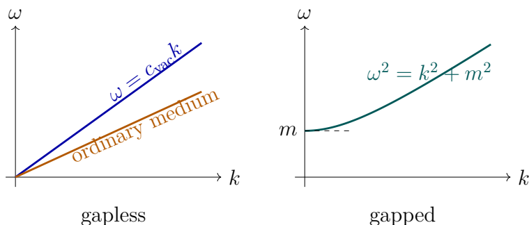
Figure 8.1: Changing the propagation speed changes the slope of a gapless dispersion relation. Giving the excitation a mass opens a nonzero gap at k = 0 .
