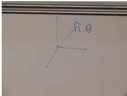
Figure 3.1: An axis \hat{\mathbf{n}} and an angle \theta specify a spatial rotation.
