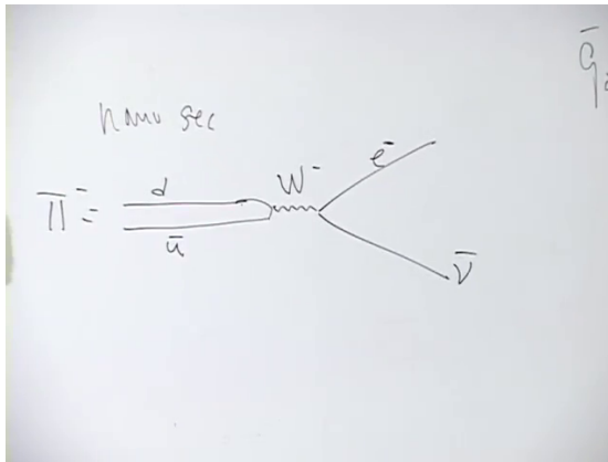
Figure 5.4: A d\bar{u} pion annihilates into a virtual W^- , followed by a charged lepton and its matching antineutrino.
