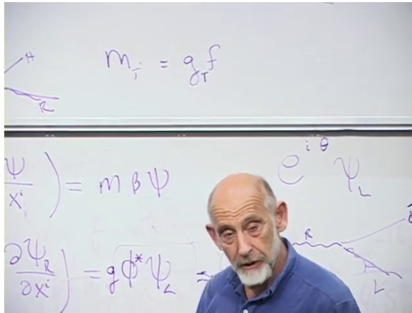
Figure 9.6: The board summarizes the species dependence as m_i = g_i f ; the g_i written there are the Yukawa couplings called y_i here.
