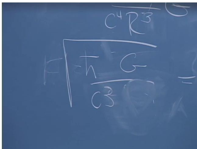
Figure 10.11: The corrected endpoint of the live dimensional check: r = \sqrt{\hbar G/c^3} .
