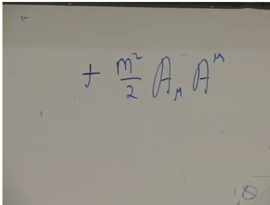
Figure 7.8: The proposed bare vector mass \frac{1}{2}m^2 A_\mu A^\mu . Its failure under A_\mu \mapsto A_\mu - \partial_\mu\theta is the obstruction that sets up the Higgs mechanism.
