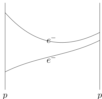
Figure 1.4: Electron exchange between two proton worldlines, understood as a schematic of quantum amplitudes rather than a watched path.
