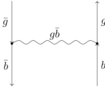
Figure 2.8: Exchange of a g\bar{b} gluon changes a blue–antiblue pair into a green–antigreen pair; antiquark arrows point opposite to increasing time.
