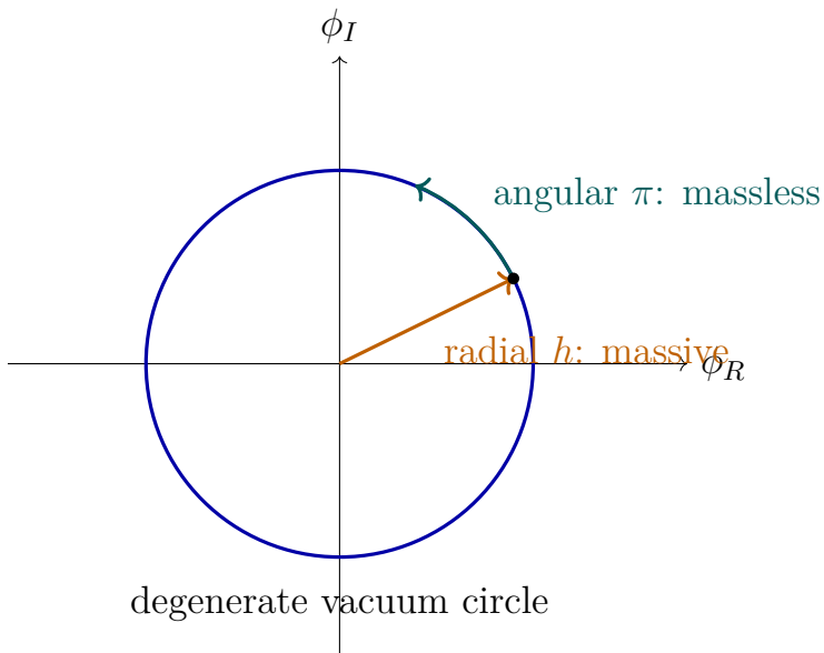
Figure 8.4: The global broken theory has curvature normal to the vacuum circle but no curvature along it. The radial Higgs mode is massive; the angular Goldstone mode is massless.
