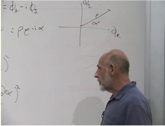
Figure 8.2: The complex scalar represented in its internal (\phi_R, \phi_I) -plane. The radius is \rho , and \alpha is the internal phase.
