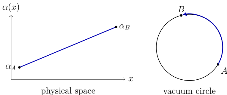
Figure 7.4: The same low-energy configuration in two descriptions. The angle varies linearly across physical space while the field follows the short arc of the vacuum circle in internal space.
