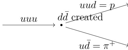
Figure 2.4: Constituent regrouping in the decay \Delta^{++} \rightarrow p + \pi^+ .
