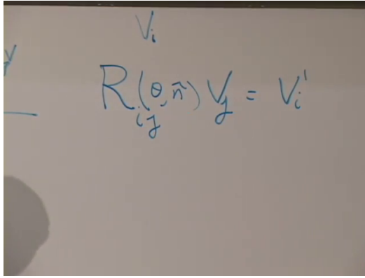
Figure 3.2: A rotation matrix maps the original vector components to the rotated components.
