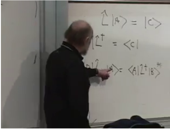
Figure 7.15: The adjoint relation obtained by reversing the bra-ket order and complex conjugating the matrix element.
