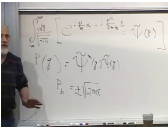
Figure 9.11: The board collects both momentum amplitudes associated with one free-particle energy.
