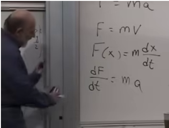
Figure 1.9: The board at 00:35:25. The deliberately phony law F = mV , its position-dependent form F(x) = m dx/dt , and the first differentiated relation are all legible.
