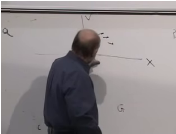
Figure 1.7: The board at 00:38:10 revisits the (x, v) phase-space plane. The horizontal x -axis and vertical v -axis are visible; the small arrows are qualitative, not a complete measured vector field.
