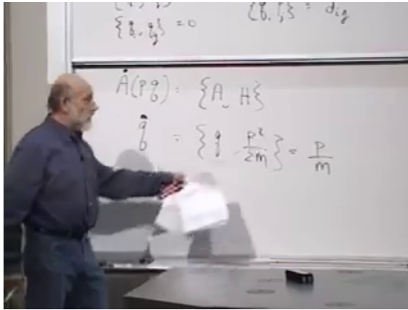
Figure 9.5: The free-particle calculation at 00:29:22. The Poisson algebra gives \dot{p} = 0 and \dot{q} = p/m directly.
