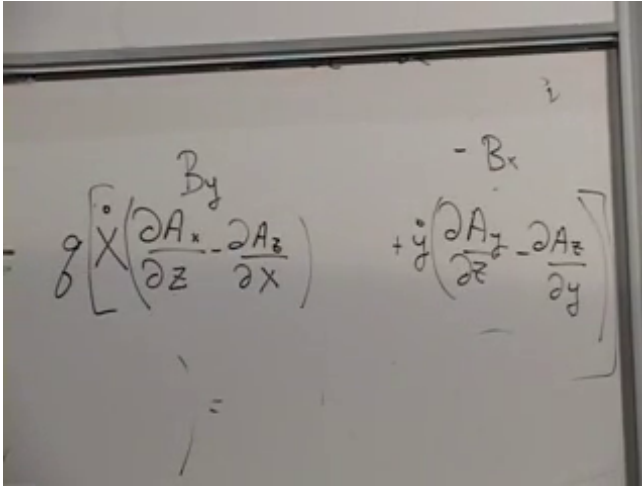
Figure 7.12: The surviving derivative combinations at 01:44:20, identified as B_y and -B_x , complete the z -component of the Lorentz force.
