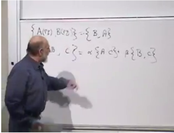
Figure 9.1: Antisymmetry and linearity on the board at 00:09:12. The minus sign in the first rule is the feature that fixes the order of every later bracket.
