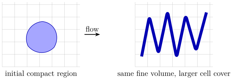
Figure 7.6: Fine-grained volume and coarse-grained coverage. Stretching and folding preserve exact volume, while finite-resolution cells can report a larger occupied region.
