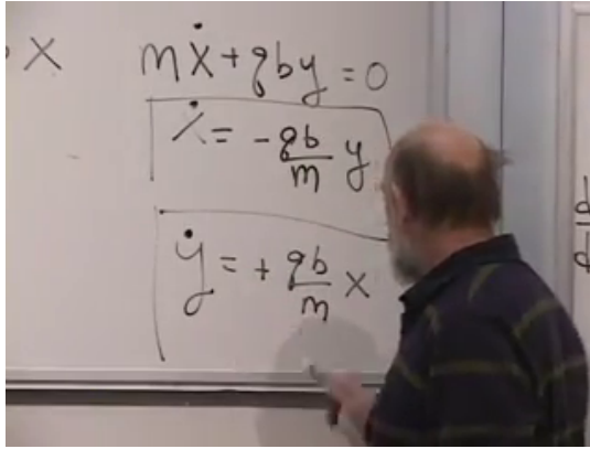
Figure 8.6: The two velocity relations together at 00:52:00. Their form already identifies uniform circular motion.
