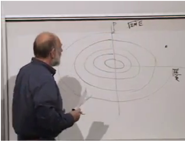
Figure 5.12: Nested constant-energy ellipses in the x - p plane at 01:40:34. The board also marks the momentum and position intercepts.
