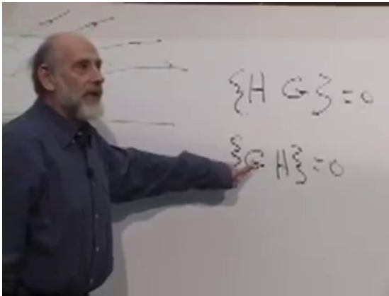
Figure 9.13: The symmetry condition at 01:05:44: \{H, G\} = 0 is equivalently \{G, H\} = 0 .
