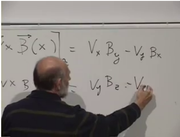
Figure 7.7: Components of \mathbf{v} \times \mathbf{B} at 01:18:40. The upper line isolates the z -component used in the derivation below.
