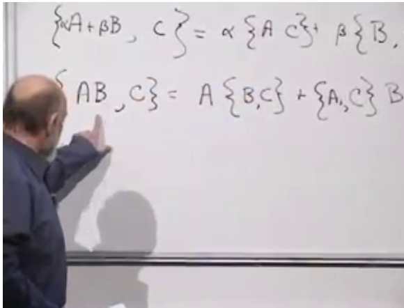
Figure 9.2: The product rule at 00:11:18. In classical mechanics the functions outside the bracket multiply as ordinary commuting numbers.
