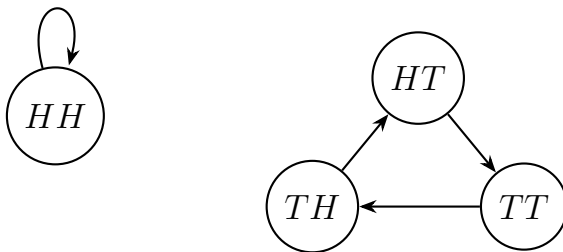
Figure 1.11: Clean reconstruction of the reversible four-state update in Eq. (1.28).
