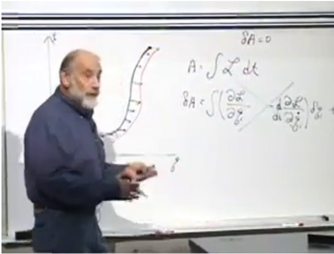
Figure 4.4: The endpoint form of the variational argument at 00:47:50. The bulk Euler–Lagrange term is crossed out because the original path obeys the equations of motion, leaving the boundary contribution whose equality at two times is the conservation law.
