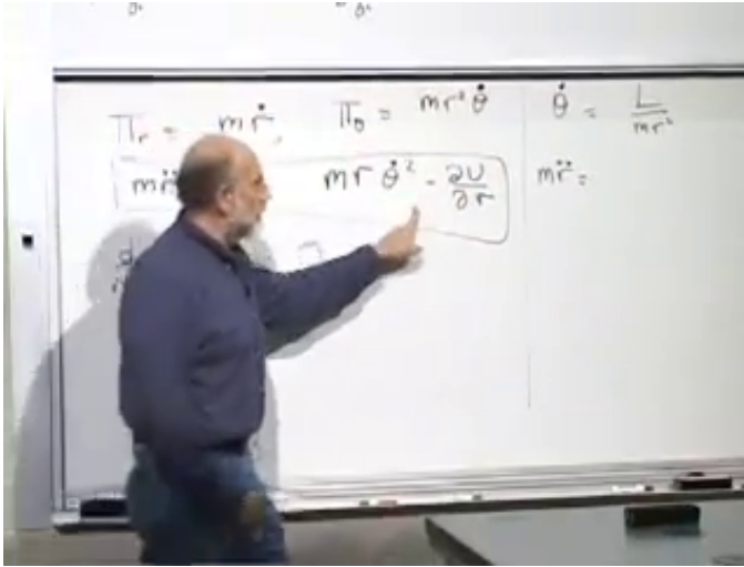
Figure 4.2: The polar equations assembled at 00:18:05. Rotational symmetry makes mr^2\dot{\theta} constant, and the same board retains the radial equation that will receive this constant as an input.
