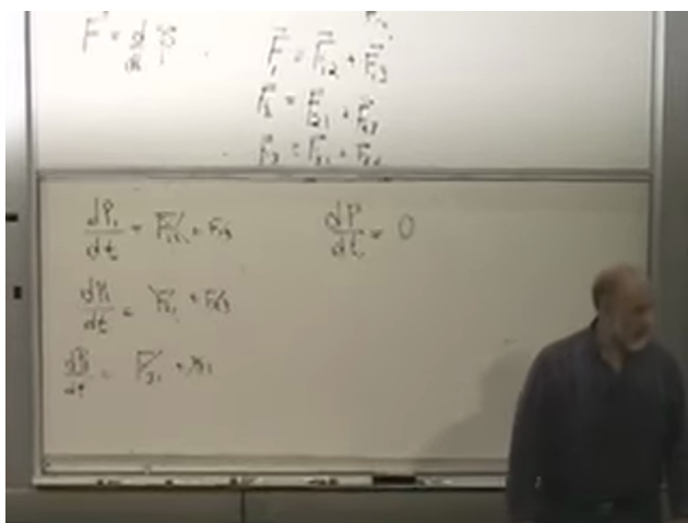
Figure 2.5: The completed cancellation board at 00:35:20. Each internal force appears once with each orientation, leaving \dot{\mathbf{P}} = 0 .
