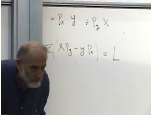
Figure 4.6: The rotational Noether charge at 01:04:10. The board identifies \sum_a (x_a p_{y_a} - y_a p_{x_a}) with angular momentum.
