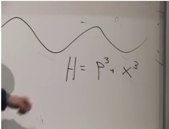
Figure 6.9: A deliberately nonstandard Hamiltonian at 01:25:50. It shows directly that the canonical momentum need not be proportional to velocity.
