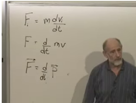
Figure 2.3: The component, scalar, and vector forms of Newton's momentum law at 00:29:00.
