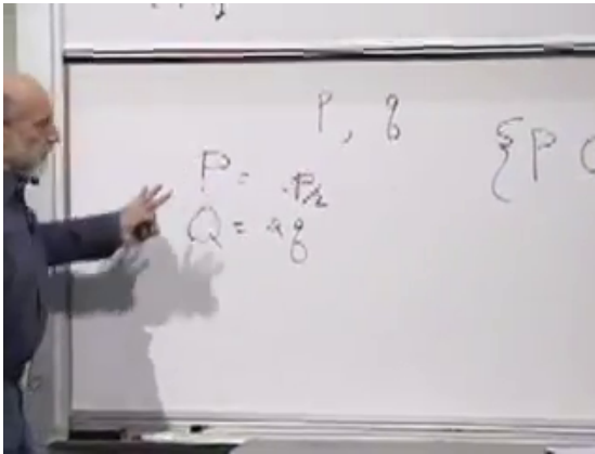
Figure 9.6: The compensated rescaling at 00:33:55. Stretching q while squeezing p preserves the canonical bracket.
