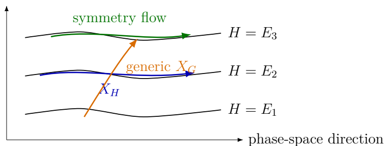
Figure 9.12: Reconstruction of the board geometry: a generic generator crosses energy surfaces, whereas a symmetry generator is tangent to them.
