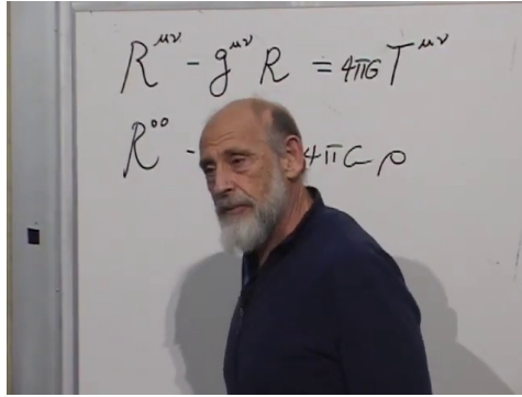
Figure 5.2: Einstein field equation and its 00 component.
