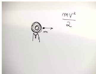
Figure 2.2: Outgoing test mass and the kinetic-energy term \frac{1}{2}mv^2 .
