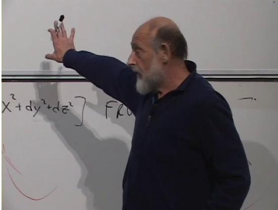
Figure 5.1: Flat FRW metric fragment.
