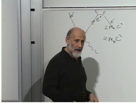
Figure 6.1: Pair-production threshold sketch comparing the electron and proton mass scales.
