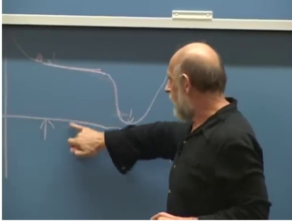
Figure 8.1: Qualitative inflaton potential with a broad plateau, a steep drop, and a low minimum.
