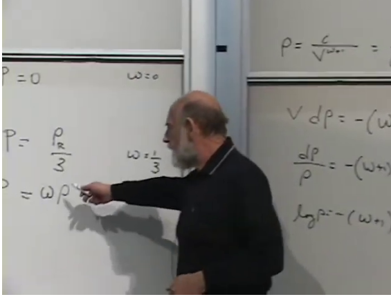
Figure 4.4: Equation of state P = \omega \rho together with the density-scaling argument.
