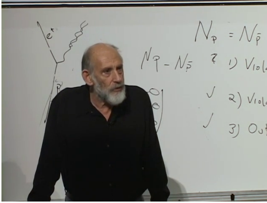
Figure 6.2: Conditions for generating a baryon asymmetry from an initially symmetric state.
