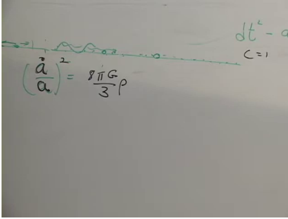
Figure 4.2: Basic expansion equation together with the one-dimensional line analogy.
