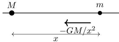
Figure 1.2: The radial one-particle problem used to separate the sign of acceleration from the direction and fate of motion.
