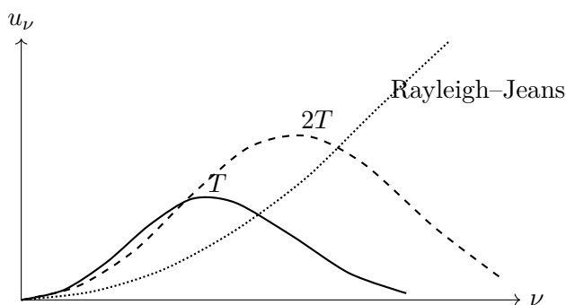
Figure 7.2: The classical spectrum rises without bound, while Planck spectra turn over. Increasing the temperature shifts the characteristic frequency upward and preserves the dimensionless shape.
