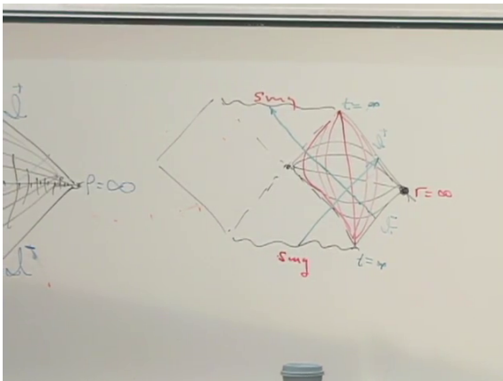
Figure 4.7: The completed eternal Schwarzschild Penrose diagram, with singularities, horizons, null trajectories, and one asymptotic boundary marked on the board.
