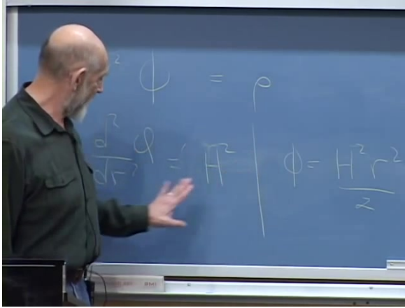
Figure 9.10: The uniform-source equation and the quadratic de Sitter potential.
