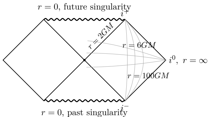
Figure 5.4: The right exterior resembles the flat wedge at large radius. Its inner null edge is r = 2GM when c = 1 ; the other labeled radii are schematic examples.
