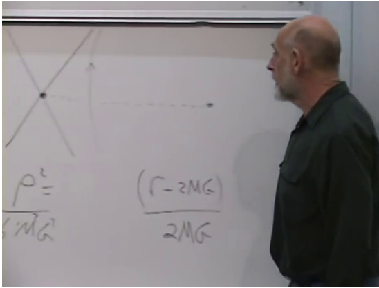
Figure 3.3: The near-horizon causal board: crossed null boundaries, constant-radius hyperbolae in the exterior wedge, and the coordinate relation between \rho and r - 2GM .
