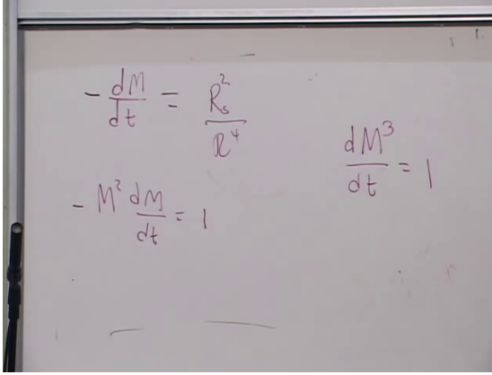
Figure 3.6: The unobstructed evaporation board: luminosity gives -dM/dt \sim 1/M^2 , hence a uniform decrease of M^3 and a lifetime proportional to the initial mass cubed.
