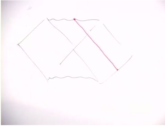
Figure 5.5: The null shell, in red, drawn across the Schwarzschild diagram while the correct exterior portion is being isolated.
