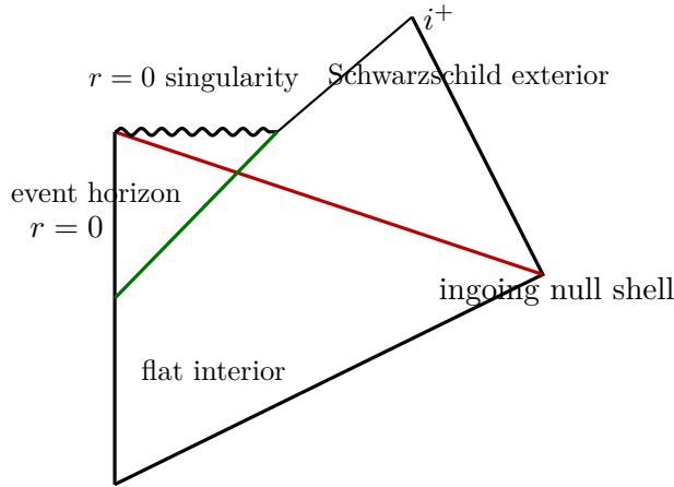
Figure 5.6: The collapse geometry. The red shell joins a flat interior to a Schwarzschild exterior. The green event horizon begins earlier in the flat region and ends at the future boundary of the black-hole region.
