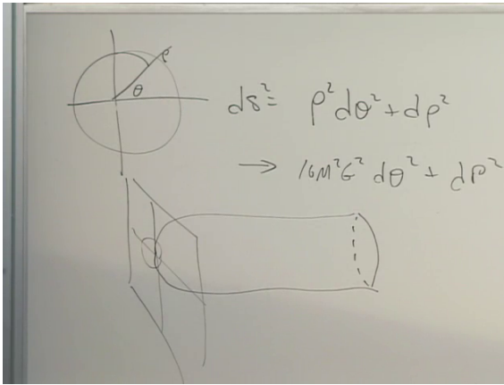
Figure 4.2: The Euclidean comparison: a polar tip joined to an asymptotic cylinder of circumference 8\pi GM .
