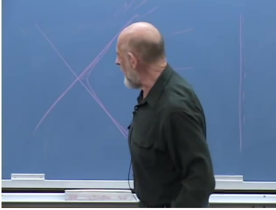
Figure 9.3: The classical horizon and the nearby stretched horizon used in the exterior description.
