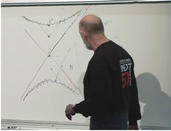
Figure 4.3: The developed causal sketch: crossed horizons, future and past singularity curves, and observer trajectories accumulated during the discussion.
