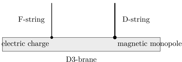
Figure 1.4: D3-brane worldvolume interpretation. An F-string endpoint appears as an electric charge; a D-string endpoint appears as a magnetic monopole.
