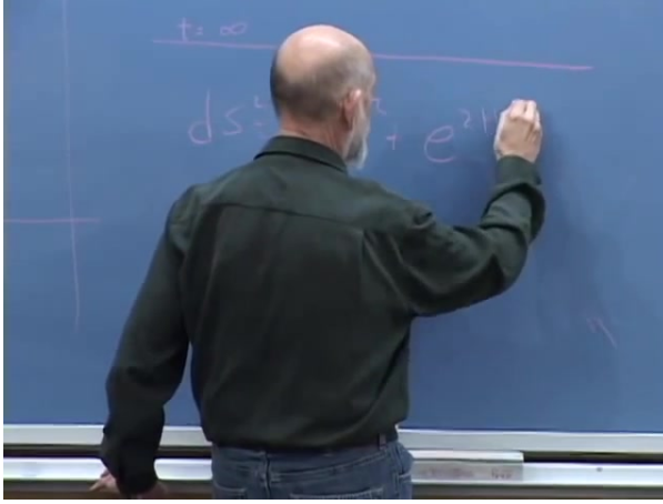
Figure 9.4: The exponentially expanding de Sitter metric in flat coordinates.
