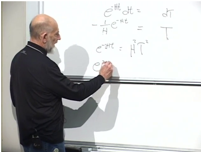
Figure 8.12: The algebra relating e^{2Ht} to 1/(H^2 T^2) , preparing the conformal form of the metric.
