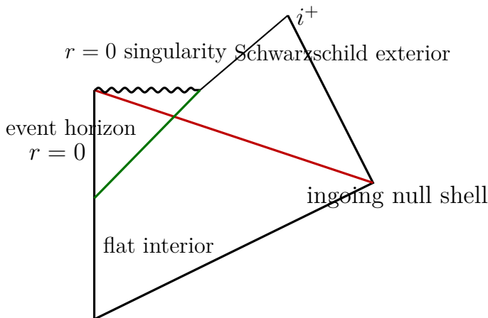
Figure 5.6: The collapse geometry. The red shell joins a flat interior to a Schwarzschild exterior. The green event horizon begins earlier in the flat region and ends at the future boundary of the black-hole region.
