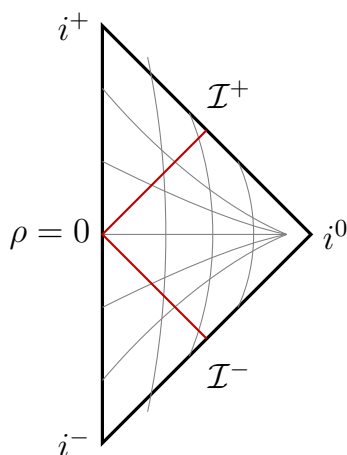
Figure 4.6: Radial Minkowski spacetime in a finite triangle. The red null ray enters from \mathcal{I}^- , reaches the origin, and leaves through \mathcal{I}^+ .
