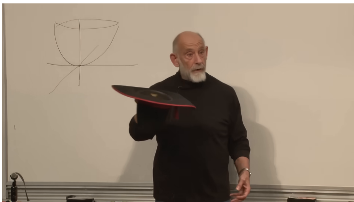
Figure 1.1: The ordinary symmetric bowl and the physical hat used to make rotational symmetry in field space tangible.
