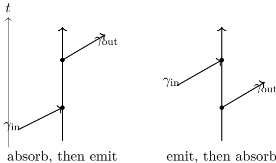
Figure 10.15: The two lowest-order time orderings for electron–photon scattering.
