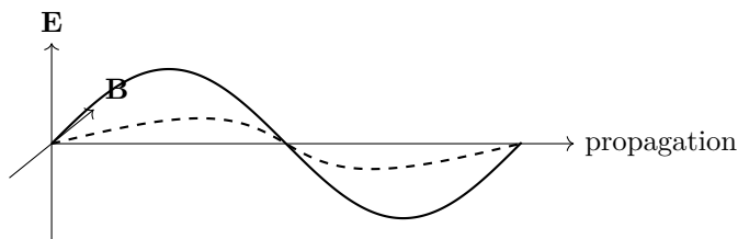
Figure 1.3: In an electromagnetic wave, the electric and magnetic fields are mutually perpendicular and both are transverse to the direction of propagation.
