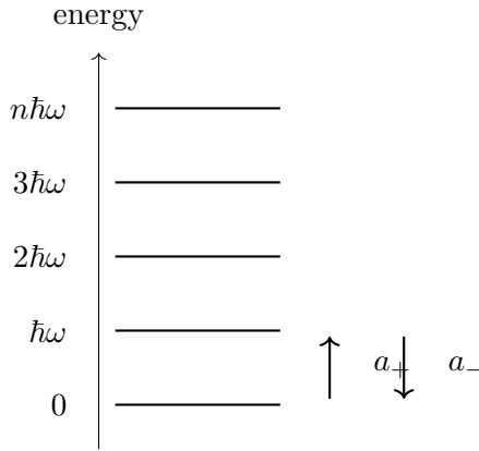
Figure 2.10: Equally spaced oscillator levels in the convention E_n = n\hbar\omega .
