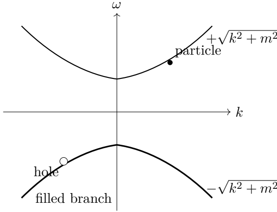
Figure 6.6: At every momentum the massive spectrum has positive- and negative-energy states. The negative branch is filled, and a missing state in it is a positive-energy hole.
