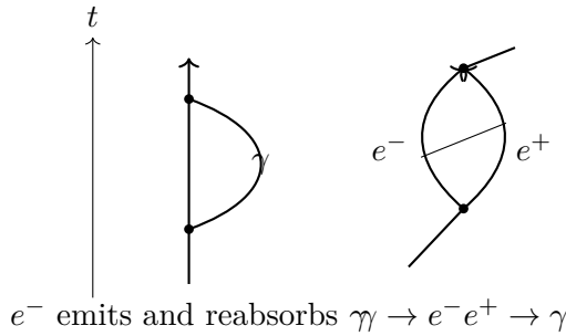
Figure 10.11: An electron self-emission contribution and a photon history containing an electron-positron pair.
