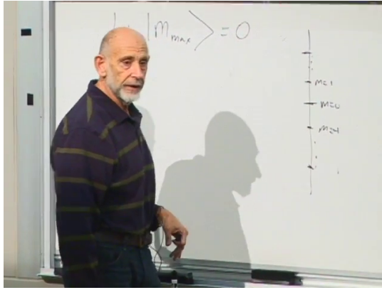
Figure 7.2: The highest-weight condition terminates the raising sequence, and the allowed m values form a finite unit-spaced ladder.
