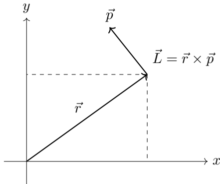
Figure 7.1: For a particle at position \vec{r} with momentum \vec{p} , the angular momentum \vec{L} = \vec{r} \times \vec{p} is perpendicular to their plane.
