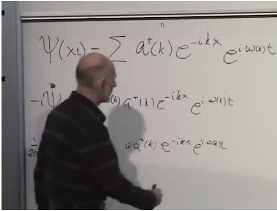
Figure 4.6: Time and spatial derivatives of the creation-field mode expansion.
