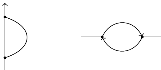
additional internal photon electron–positron insertion
