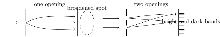
Figure 1.2: A single aperture produces a broadened image, while two apertures produce alternating constructive and destructive interference.
