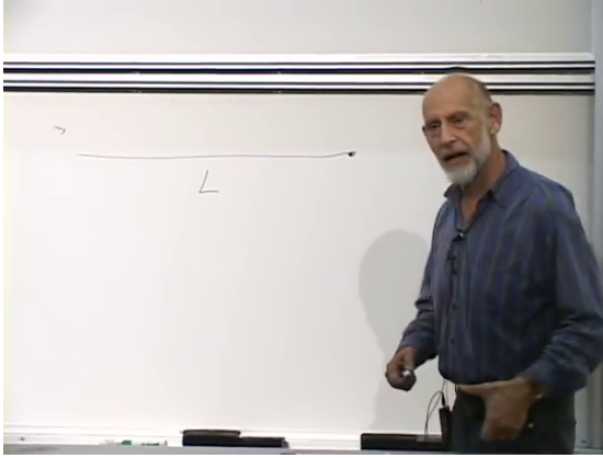
Figure 2.8: A one-dimensional path of total length L used to introduce periodic identification.
