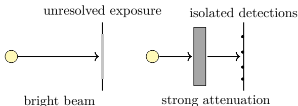
Figure 1.6: Progressive attenuation lowers the detection rate until a continuous-looking exposure resolves into isolated photon events.
