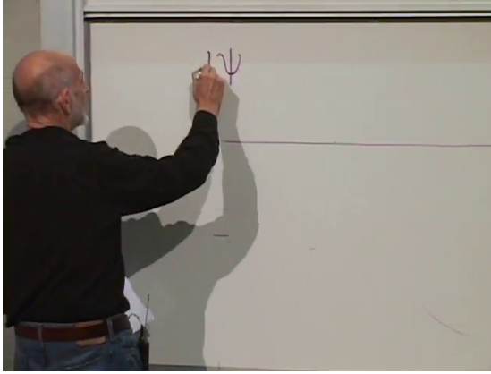
Figure 5.6: Beginning the first-order field equation whose plane waves satisfy \omega = k .
