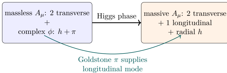
Figure 8.9: The Higgs mechanism rearranges, rather than destroys, physical degrees of freedom.
