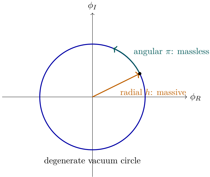
Figure 8.4: The global broken theory has curvature normal to the vacuum circle but no curvature along it. The radial Higgs mode is massive; the angular Goldstone mode is massless.
