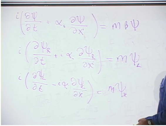
Figure 9.4: The board first writes the Dirac equation, then splits it into coupled left- and right-handed equations.
