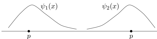
Figure 1.2: The two localized profiles used to form the equilibrium superposition after tunneling is allowed.
