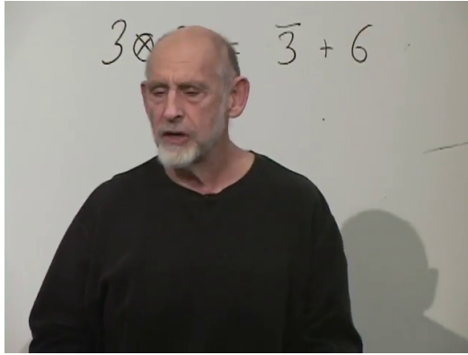
Figure 4.3: The two-quark product split into an anti-triplet and a sextet.
