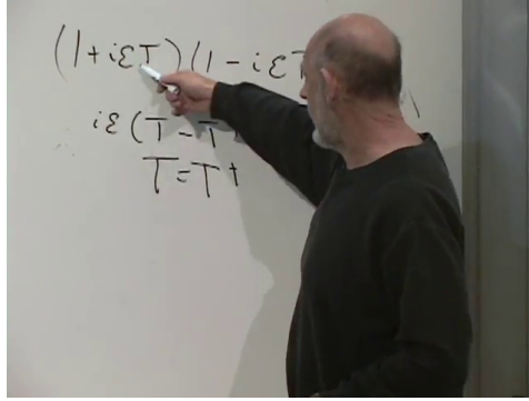
Figure 4.1: The near-identity unitarity calculation ending in T = T^\dagger .
