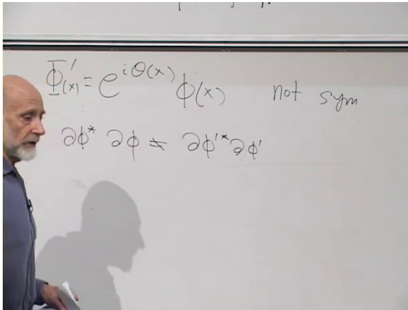
Figure 8.5: The board records the local phase transformation and the failure of the ordinary derivative term to remain invariant.
