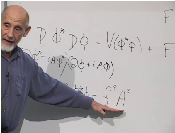
Figure 8.7: The board isolates the f^2A^2 contribution inside (D\phi)^*(D\phi) . Numerical factors depend on how the scalar field and the gauge coupling are normalized; with Eqs. (8.13) and (8.19), the result is m_A = gf .
