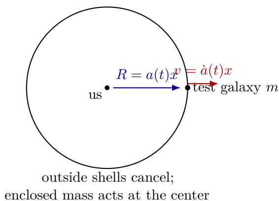
Figure 8.9: Clean reconstruction of the Newtonian construction.
