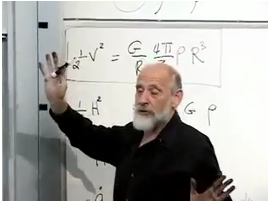
Figure 8.20: The board places the boxed Newtonian energy equation above the corresponding Friedmann equation. Source frame at 01:44:42.
