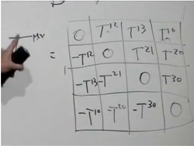
Figure 5.8: A completed antisymmetric 4 \times 4 array: zeros on the diagonal and opposite signs across it.
