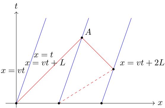
Figure 1.5: Light signals determine the moving frame's line of simultaneity.
