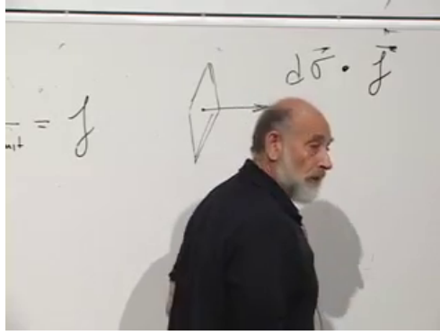
Figure 2.10: An oriented area element and the flux factor d\vec{\sigma} \cdot \vec{J} .
