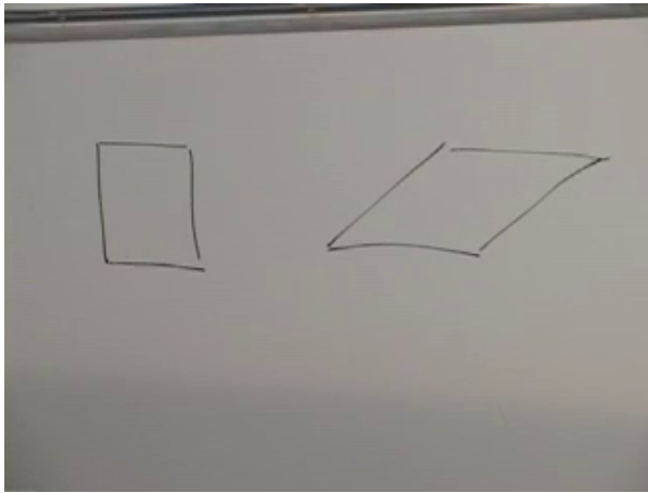
Figure 7.1: A square and its sheared image at 00:13:16. Hamiltonian flow need not preserve lengths or angles; the relevant invariant is phase-space area.
