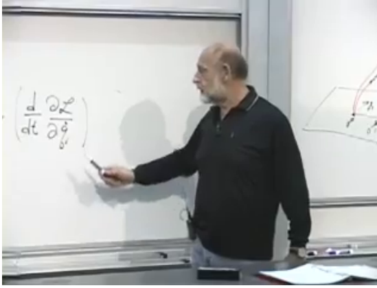
Figure 3.6: The Euler–Lagrange time-derivative term at 00:45:02, beside the trajectory picture used to connect the global path with its local equation.
