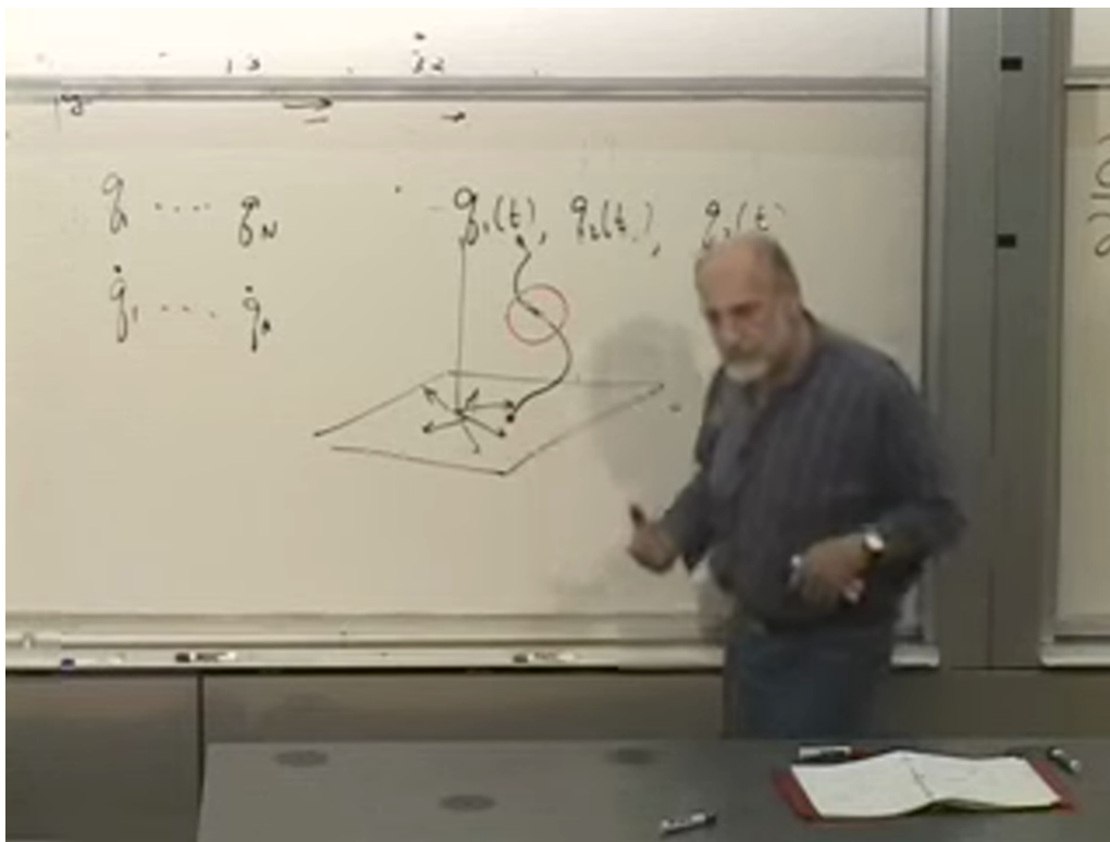
Figure 1.9: The generalized trajectory at 01:00:20. The horizontal plane stands for the many-dimensional configuration coordinates; the vertical direction represents time.
