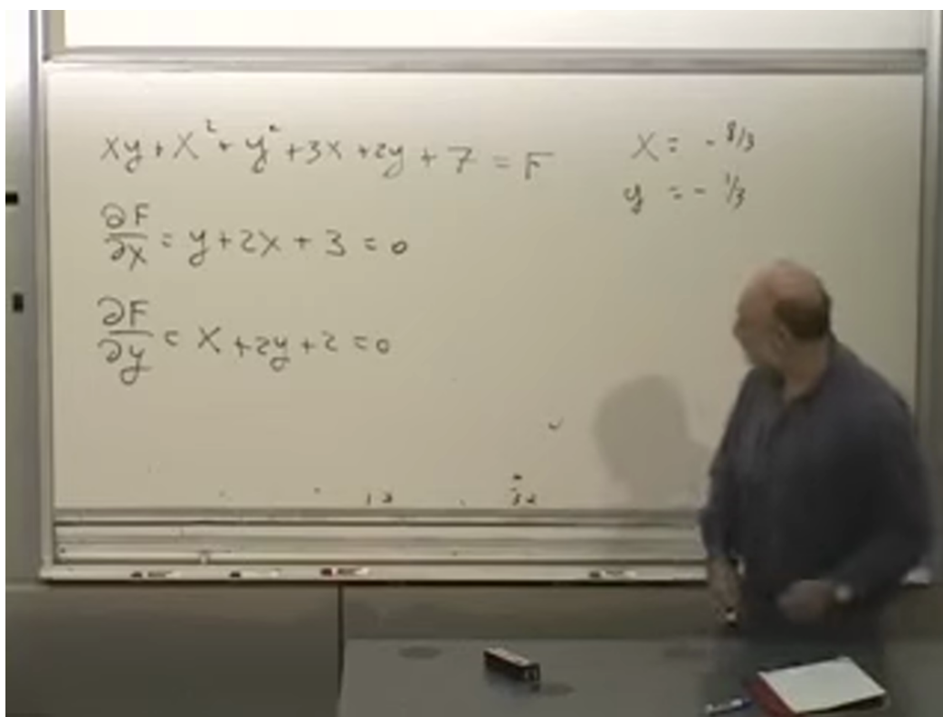
Figure 1.8: The two-variable example at 00:51:10. The displayed derivative equations are correct; the board's x = -8/3 is an arithmetic slip. Solving those equations gives Eq. (1.33).
