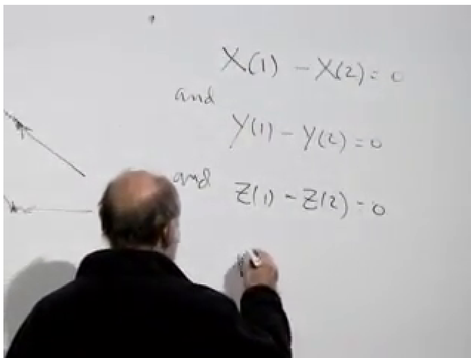
Figure 5.1: The three coordinate equalities that make collision mean spatial coincidence rather than coincidence along one preferred axis.
