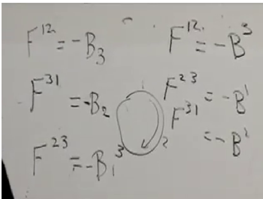
Figure 5.10: The cyclic spatial components that encode the magnetic field in the antisymmetric tensor.
