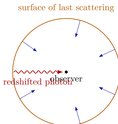
Figure 8.19: Clean reconstruction of the last-scattering picture.
