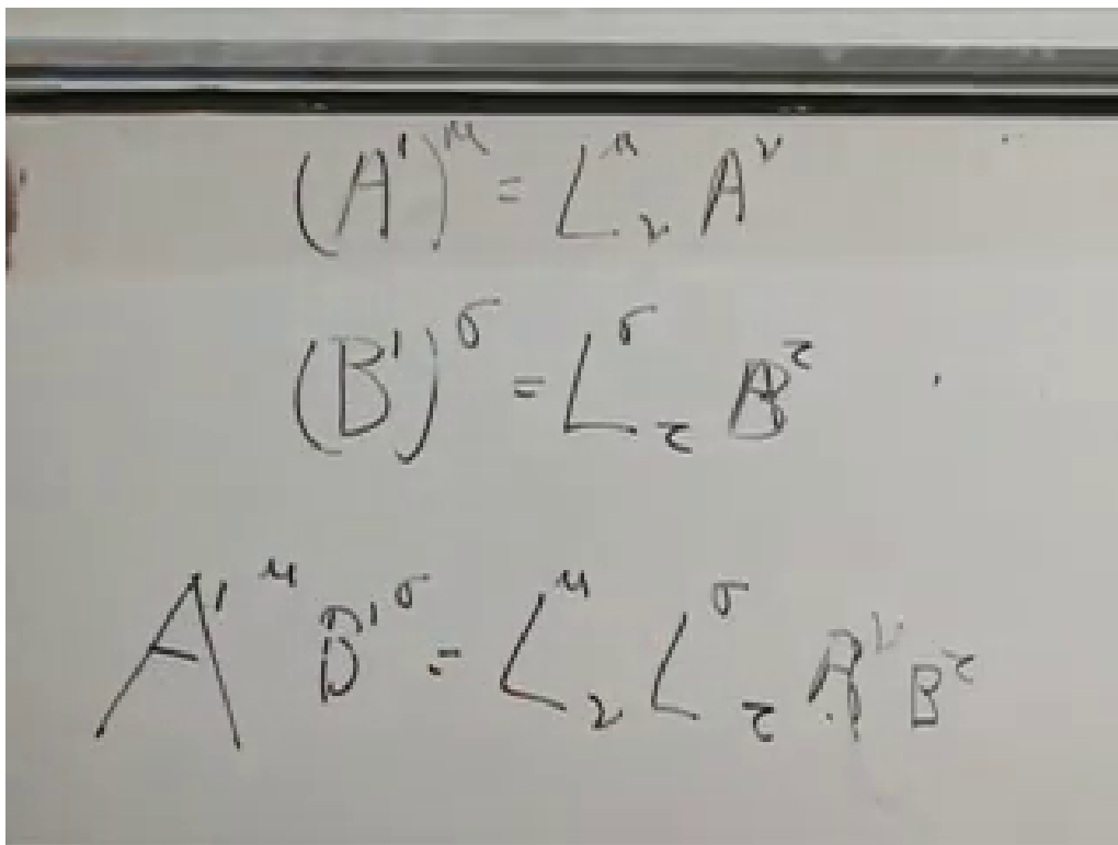
Figure 5.7: The transformation of two vectors and the resulting two-matrix transformation law for a rank-two tensor.
