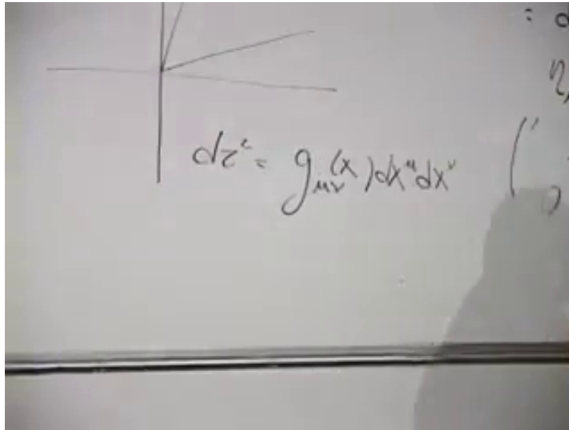
Figure 7.6: The general position-dependent metric after the coordinate grid is allowed to vary from point to point.
