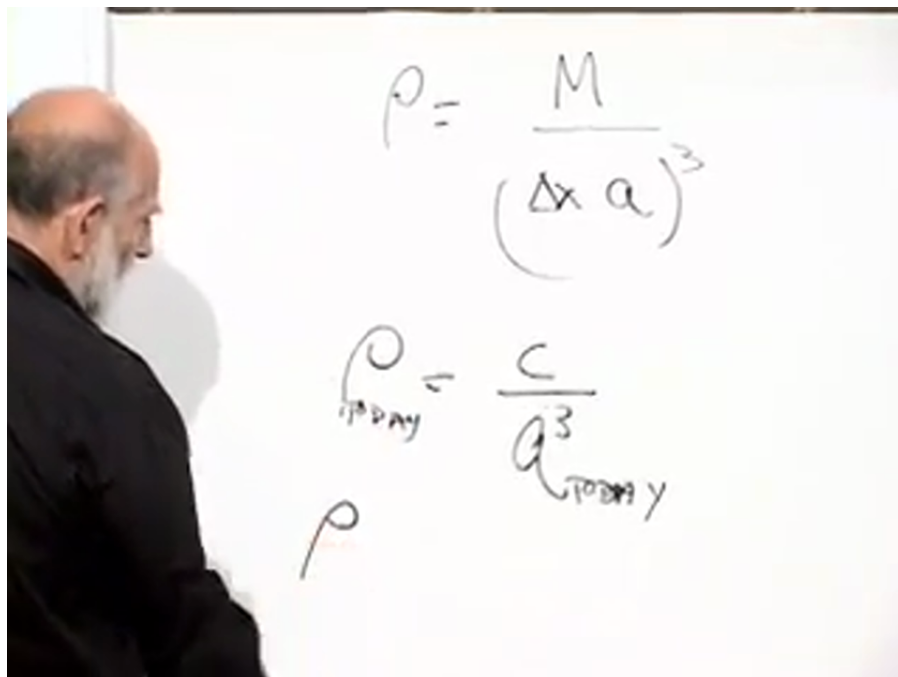
Figure 8.13: Matter density, its a^{-3} dilution, and present-day normalization. Source frame at 01:04:47.940.
