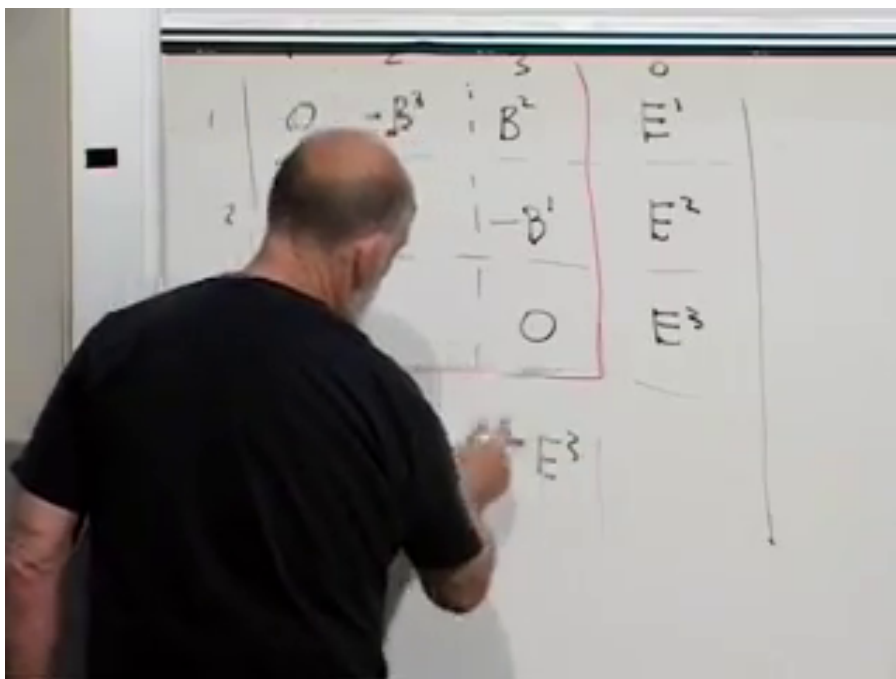
Figure 6.9: The magnetic spatial block and electric time-space column being assembled into the four-dimensional field tensor.
