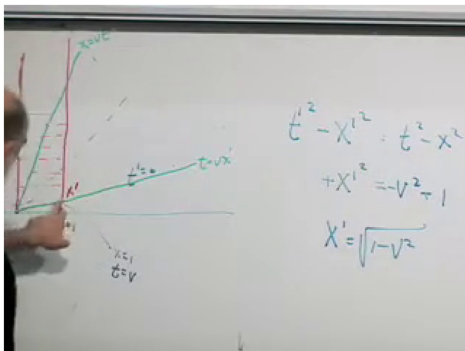
Figure 3.13: The completed length-contraction construction and the board result x' = \sqrt{1 - v^2} for a unit rest length.
