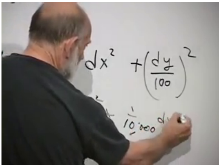
Figure 7.4: A flat plane described with centimeters on one axis and meters on the other. The unequal metric coefficients encode units, not curvature.
