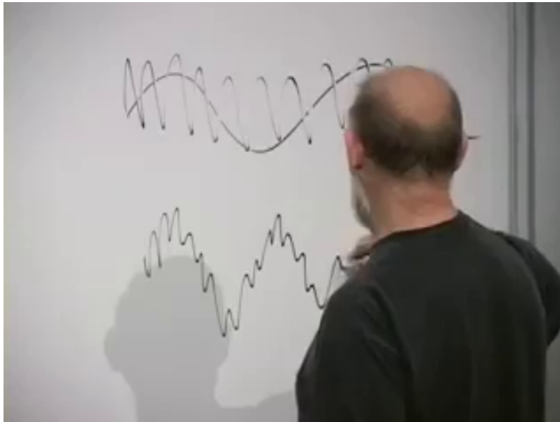
Figure 7.1: Two wave profiles on the board during the discussion of superposition. Their sum is again an allowed source-free wave.
