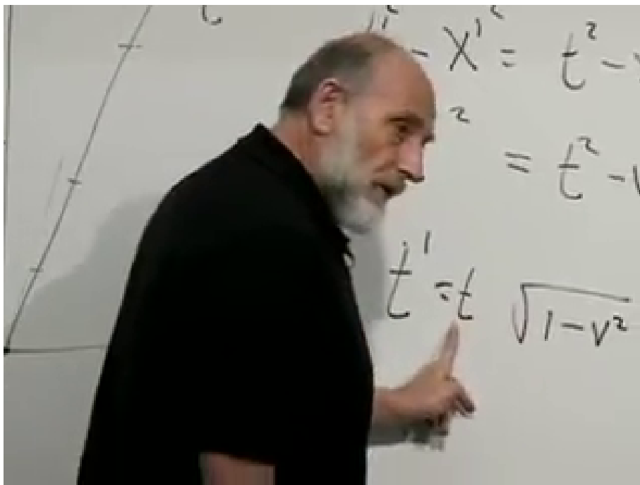
Figure 3.7: The time-dilation result on the board: the moving clock accumulates t' = t\sqrt{1-v^2} in units with c = 1 .
