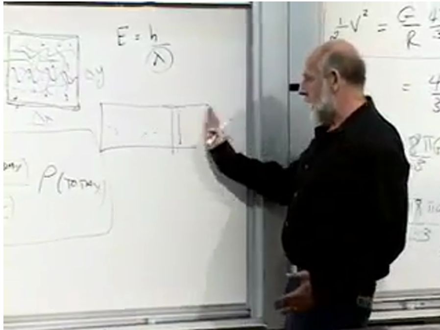
Figure 8.21: The movable photon-filled piston used to visualize pressure work. Source frame at 01:46:40.
