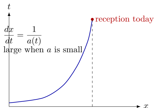
Figure 7.19: Clean version of the light-ray construction in comoving coordinates. The changing slope is a coordinate effect, not a changing local speed of light.
