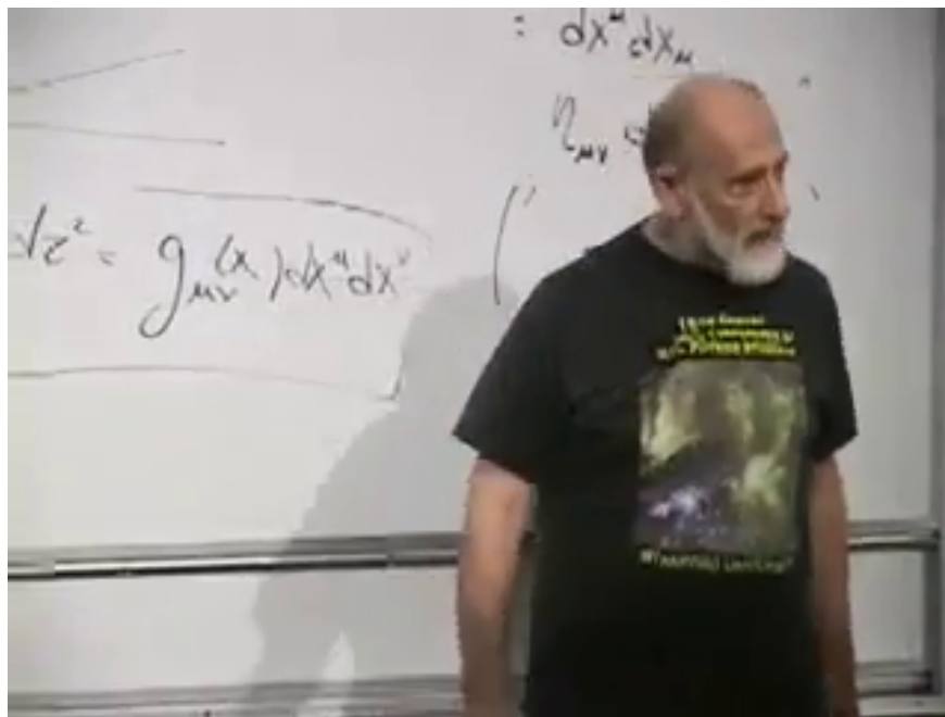
Figure 7.10: The transition from special coordinate examples to the general spacetime line element ds^2 = g_{\mu\nu}(x)dx^\mu dx^\nu .
