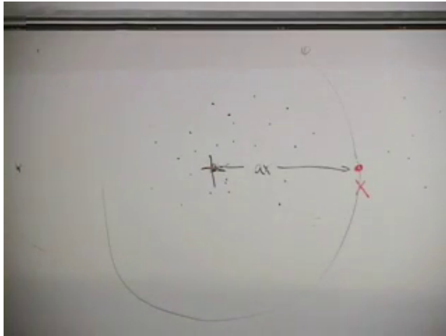
Figure 7.16: The homogeneous galaxy distribution, a test galaxy at comoving label x , and the sphere whose enclosed mass alone controls its radial motion.
