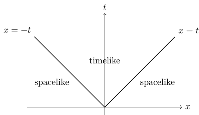
Figure 3.5: The board light cone and a clean classification of timelike, lightlike, and spacelike separation.
