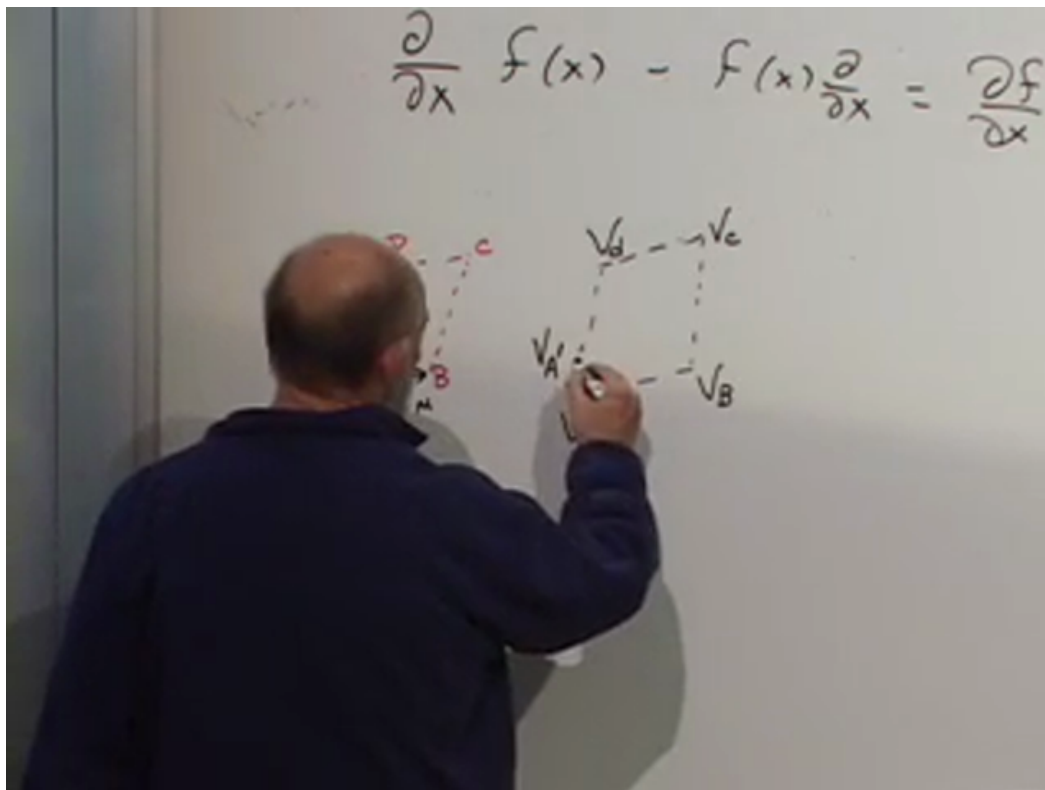
Figure 1.5: The infinitesimal loop and the values V_A, V_B, V_C, V_D, V'_A of the transported vector. The dashed mismatch at A represents a change of orientation, not a failure of the path to close.
