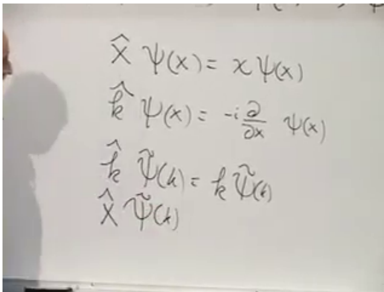
Figure 1.6: Multiplication and differentiation exchange roles in the x - and k -representations.
