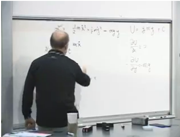
Figure 3.11: The completed near-Earth Lagrangian and coordinate derivatives at 01:19:15. The absence of x gives horizontal momentum conservation, while \partial U/\partial y = mg gives downward acceleration.
