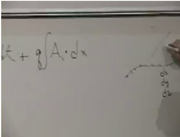
Figure 7.9: The action as a kinetic term plus a line integral of the vector potential at 01:28:50. The small path sketch emphasizes that the second term depends on the route through space.
