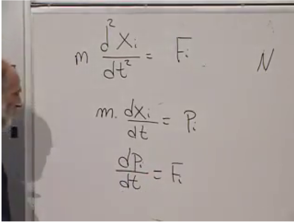
Figure 6.2: The Newton equation rewritten as two first-order equations at 00:18:48. No new physics has been added; the complete state has been made explicit.
