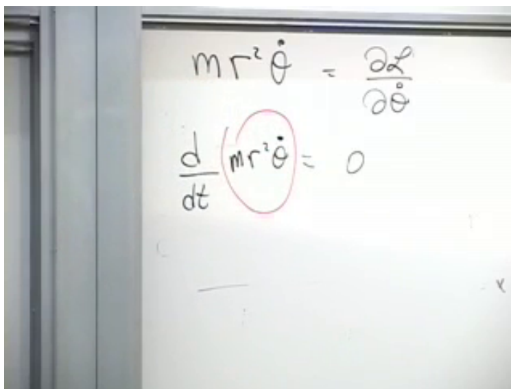
Figure 3.13: Angular momentum conservation completed on the board at 01:33:35: \frac{d}{dt}(mr^2\dot{\theta}) = 0 .
