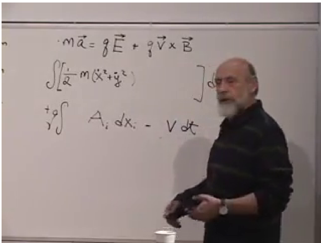
Figure 8.2: The electromagnetic action at 00:22:37. The magnetic coupling is a line integral q \int \mathbf{A} \cdot d\mathbf{x} , which becomes q\mathbf{A} \cdot \mathbf{v} in the Lagrangian.
