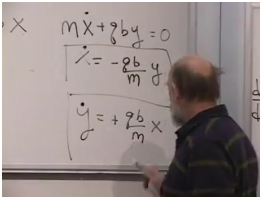
Figure 8.6: The two velocity relations together at 00:52:00. Their form already identifies uniform circular motion.
