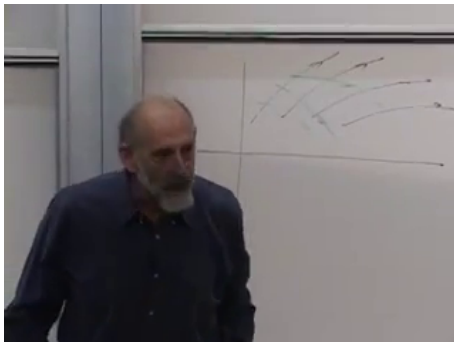
Figure 9.11: The phase-space flow picture at 01:02:10. The curved trajectories represent Hamiltonian motion; a second flow is a symmetry when it remains on the same energy surface.
