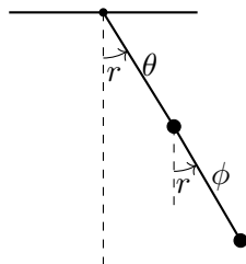
Figure 5.4: Both angles are measured from the same vertical direction. This choice makes a common rotation appear as equal shifts of \theta and \phi .
