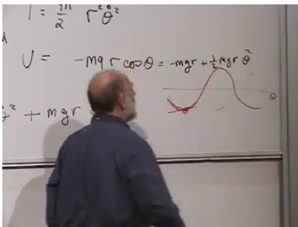
Figure 5.8: The exact pendulum potential and its quadratic approximation at 00:59:15. The parabola agrees with the cosine potential near the stable minimum and departs from it for larger angles.
