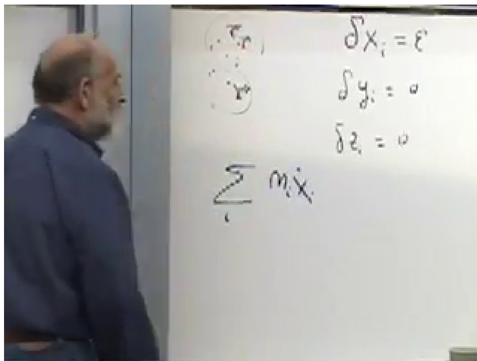
Figure 4.5: Translation along x at 00:57:30. Every particle has \delta x_a = \epsilon , while the conserved charge is the summed x -momentum \sum_a m_a \dot{x}_a .
