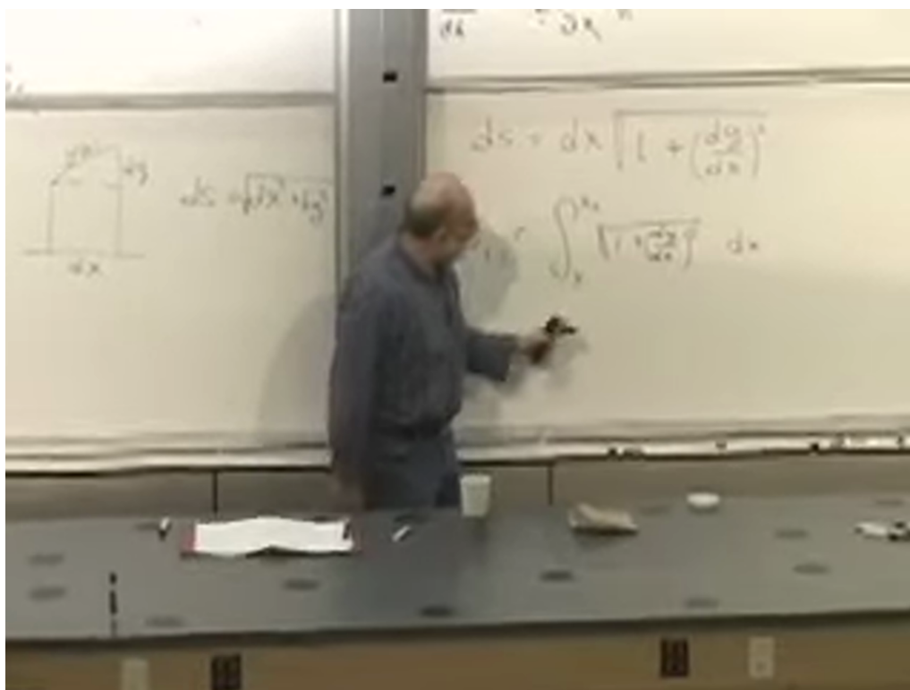
Figure 2.10: The curve, its dx - dy triangle, and the arc-length integral at 01:12:00.
