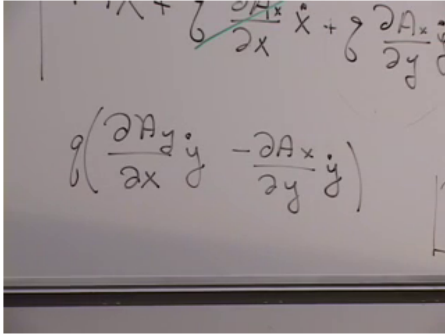
Figure 8.3: The surviving curl combination at 00:38:20. The separate derivatives of \mathbf{A} combine into the gauge-invariant field B_z .
