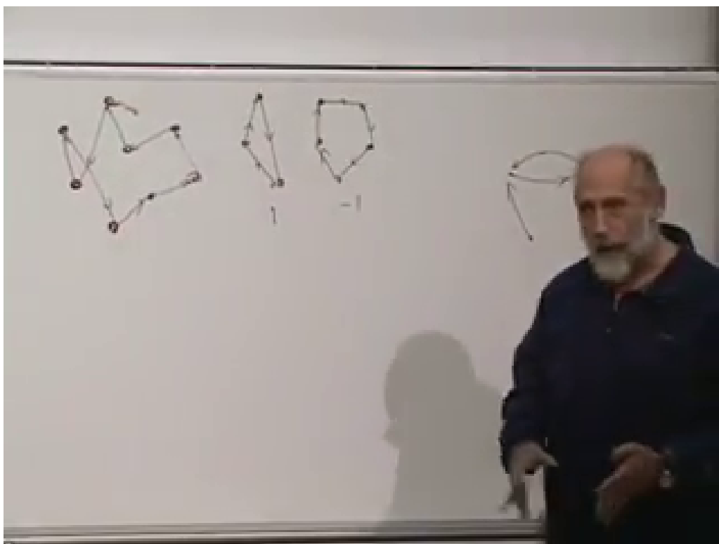
Figure 6.1: Discrete evolution at 00:08:05. The central cycles belong to separate sectors, while the map at the left illustrates how several distinct histories can merge when backward evolution is not unique.
