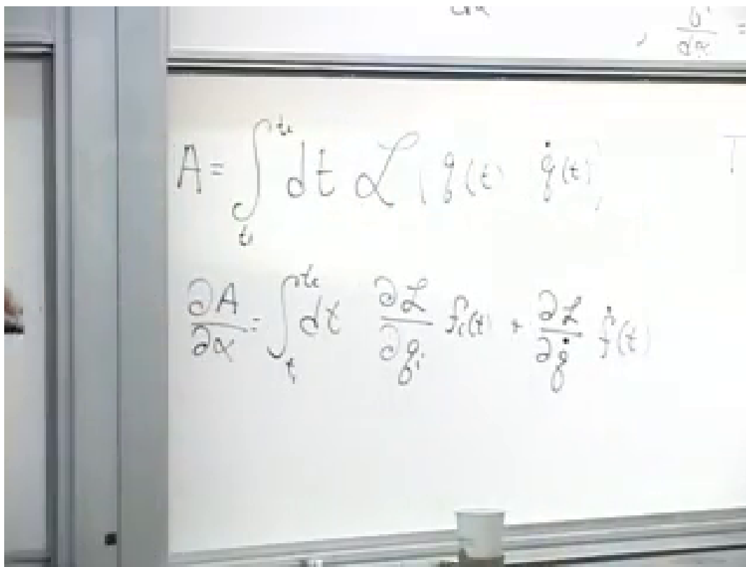
Figure 3.5: The first variation at 00:34:10. Changes of both q_i and \dot{q}_i contribute, and the audience supplies the required sum over coordinates.
