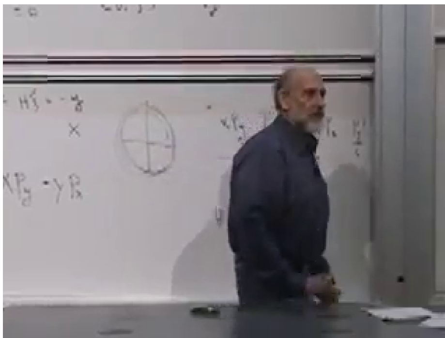
Figure 9.16: The circular orbit drawn at 01:16:35 after choosing angular momentum itself as the Hamiltonian.
