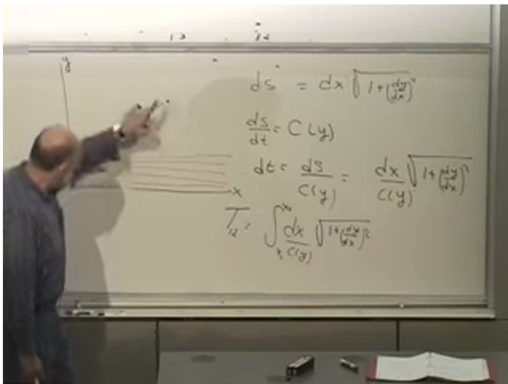
Figure 2.11: The layered-medium ray and completed least-time functional at 01:23:10. The ray bends toward the faster region while still advancing toward its endpoint.
