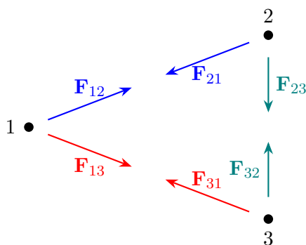
Figure 2.6: Pairwise internal forces cancel when the momentum equations for a closed system are summed.
