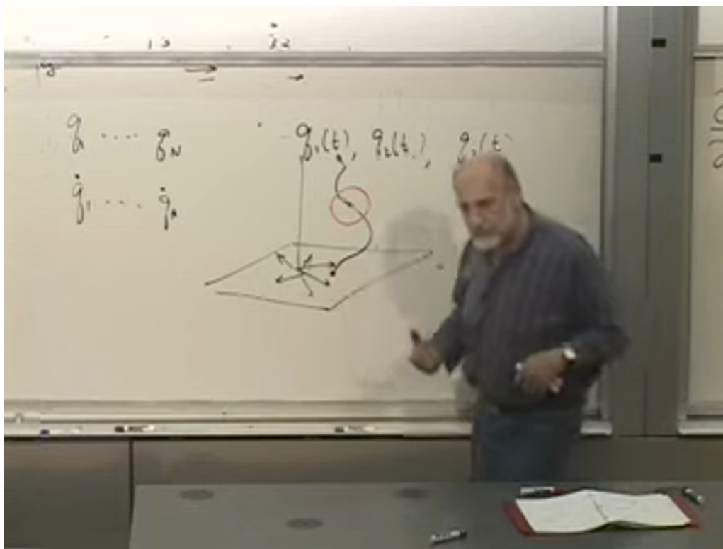
Figure 2.9: The generalized trajectory at 01:00:20. The horizontal plane stands for the many-dimensional configuration coordinates; the vertical direction represents time.
