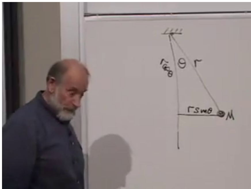
Figure 5.1: The pendulum geometry at 00:05:32. The rod length r , angle \theta , and horizontal projection r \sin \theta are complete and unobstructed.
