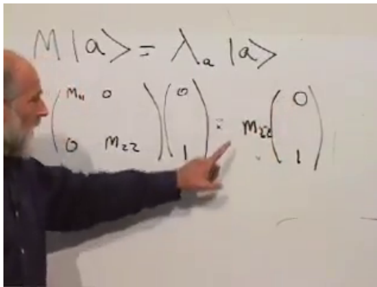
Figure 3.3: The lower basis vector returns multiplied by the lower diagonal entry.
