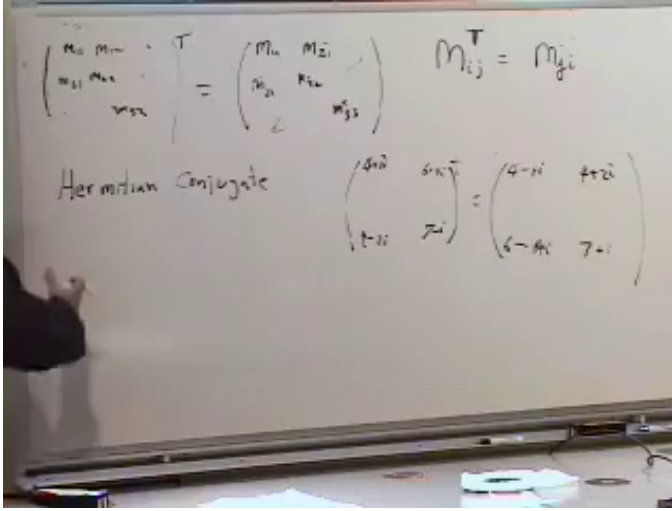
Figure 3.1: Transpose, symmetry, and the transition to Hermitian conjugation share one blackboard layout.
