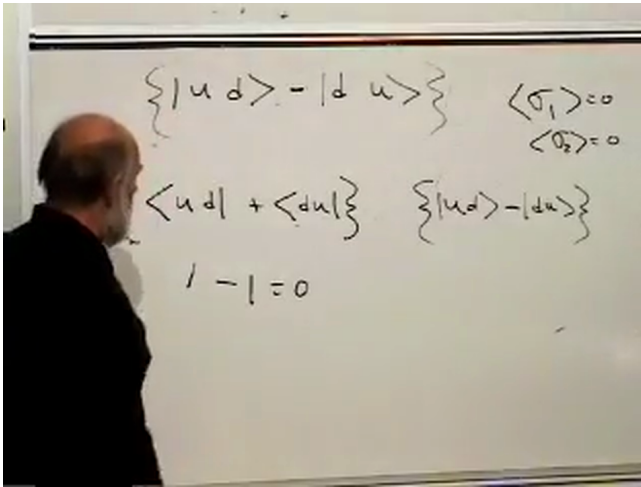
Figure 4.11: The final blackboard change replaces the symmetric superposition by the minus-sign singlet while retaining zero local spin.
