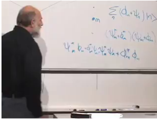
Figure 6.14: The screen amplitude and its four-term probability expansion on the board.
