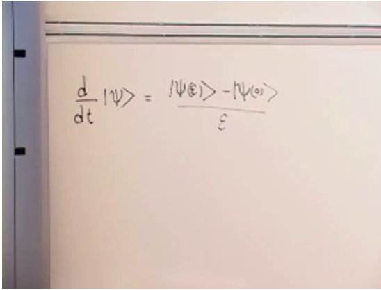
Figure 9.1: The difference quotient that turns infinitesimal evolution into a differential equation.
