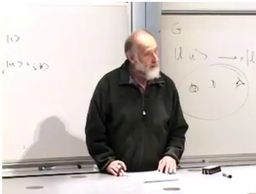
Figure 1.8: The conceptual transition from a specified ket to an ensemble description.
